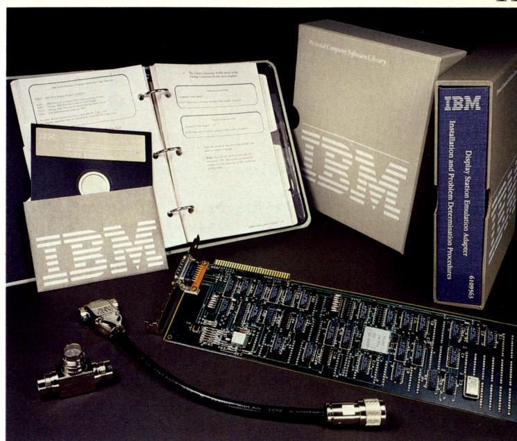
Convenience Kits provide the link between host and terminal.
