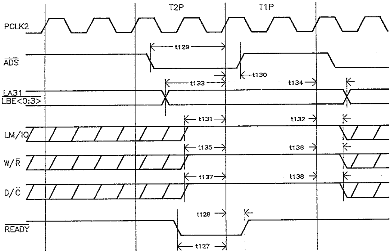
Figure 2.17 321 Input Timing
