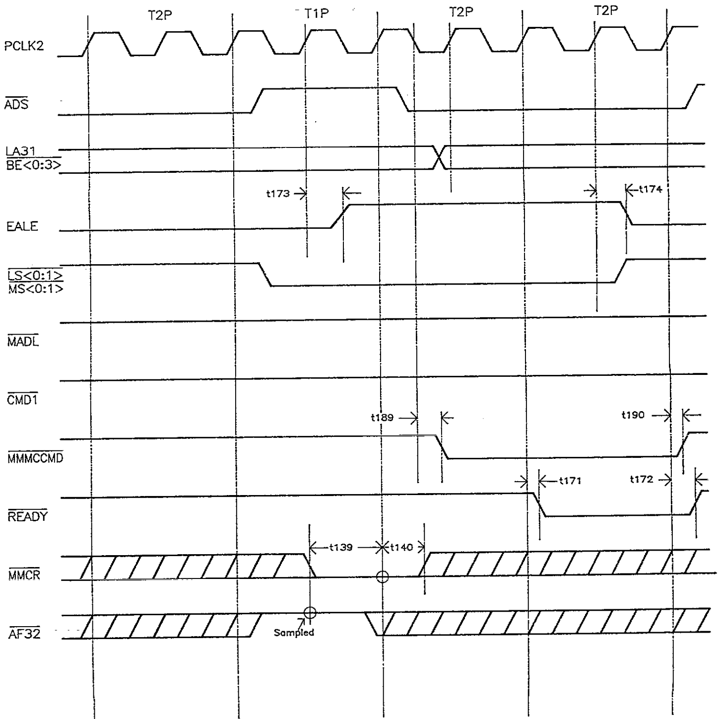
Figure 2.6 16MHz Matched Memory Cycle
