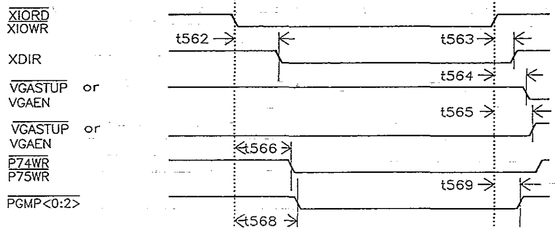
Figure 6.6 Misc. Signal Timing
