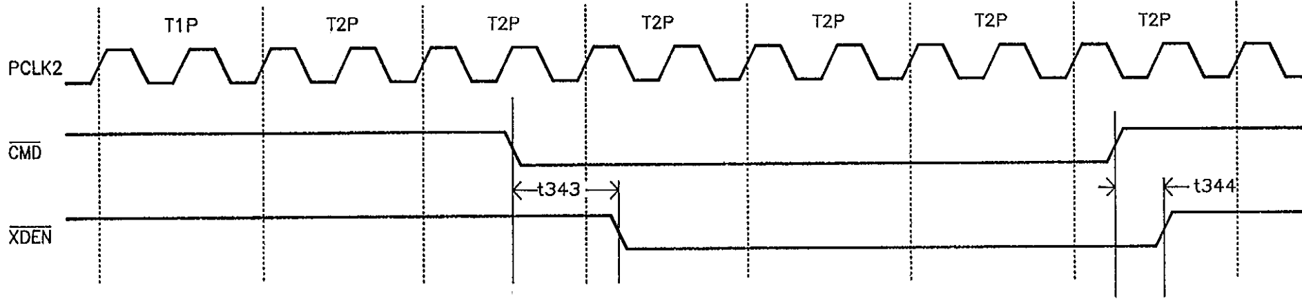
Figure 4.16 XDEN Timing
