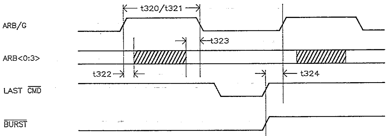
Figure 8.3 ARBITRATION TIMING
