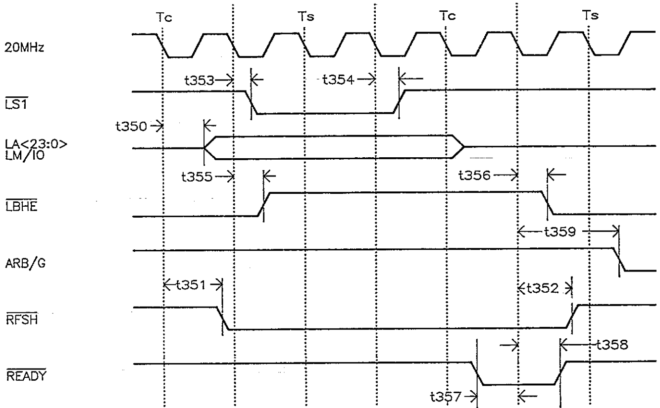
Figure 8.2 REFRESH TIMING
