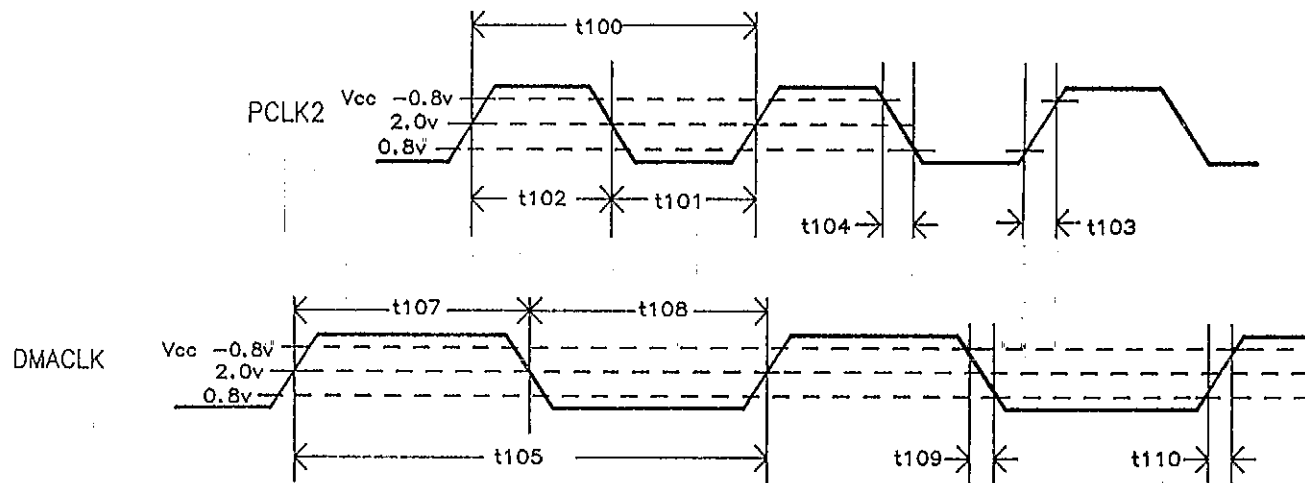
Figure 2.19 Clock Timing
