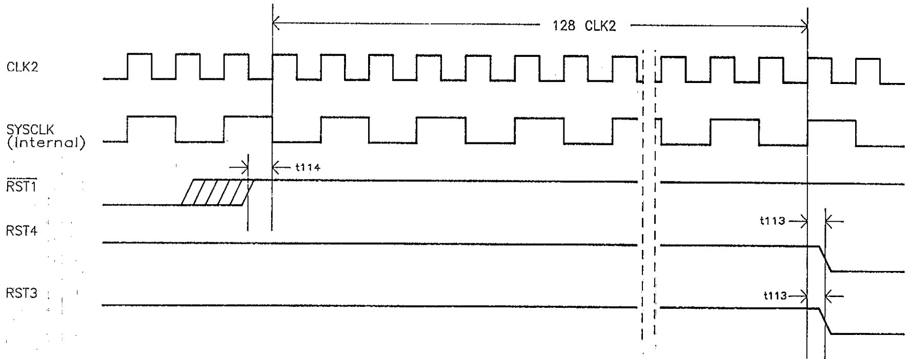
Figure 2.18 Reset 1, Reset 3 and Reset 4 Timing
