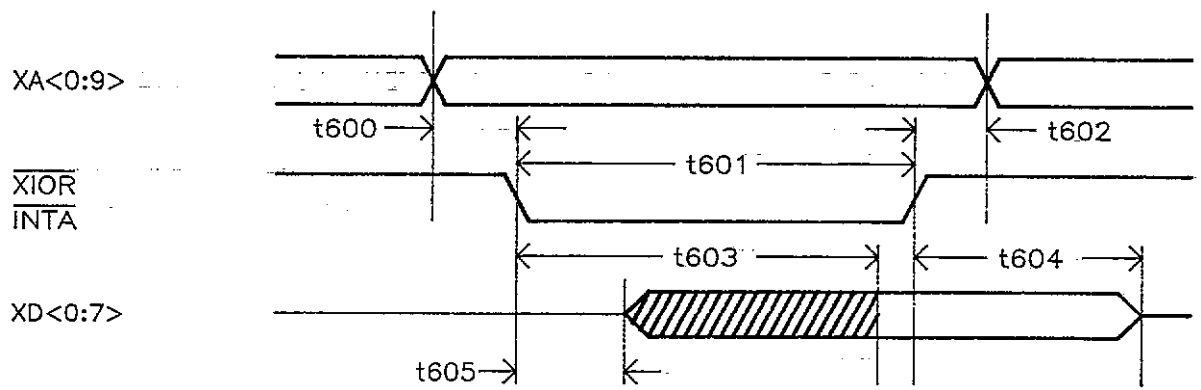
Figure 10.1 226 PERIPHERAL READ/INTA CYCLE
