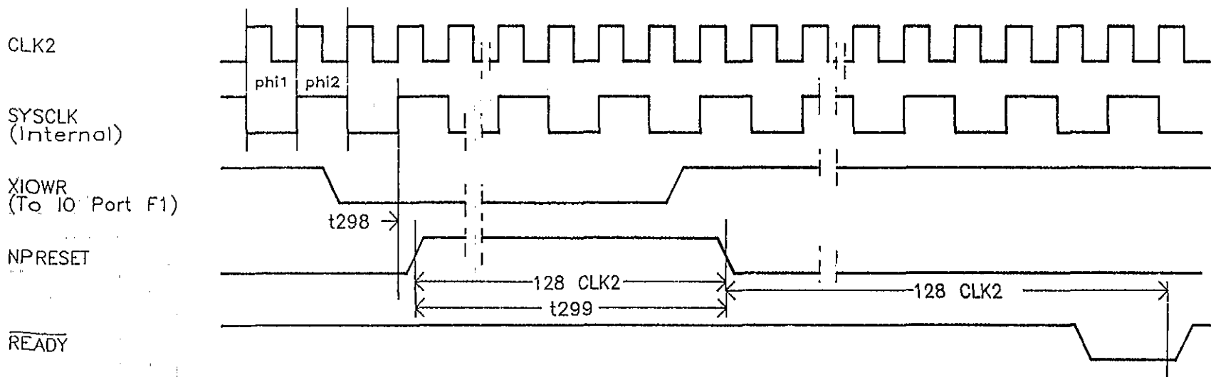
Figure 2.11 Numeric Processor Reset Timing
