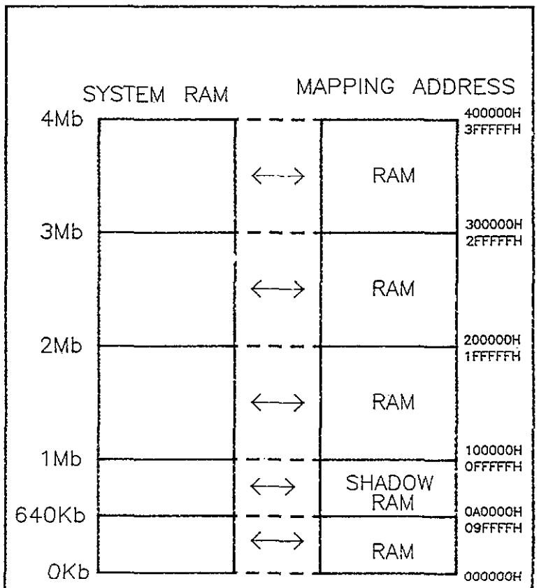
Figure 3.7 RAM Mapping with Shadow RAM (More Than 1MB of RAM)
