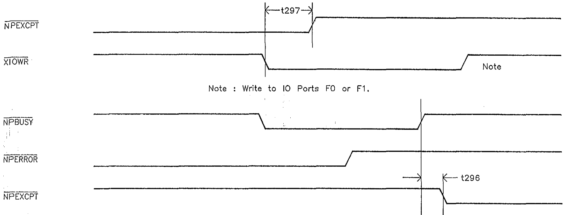
Figure 2.10 Numeric Processor Cycle
