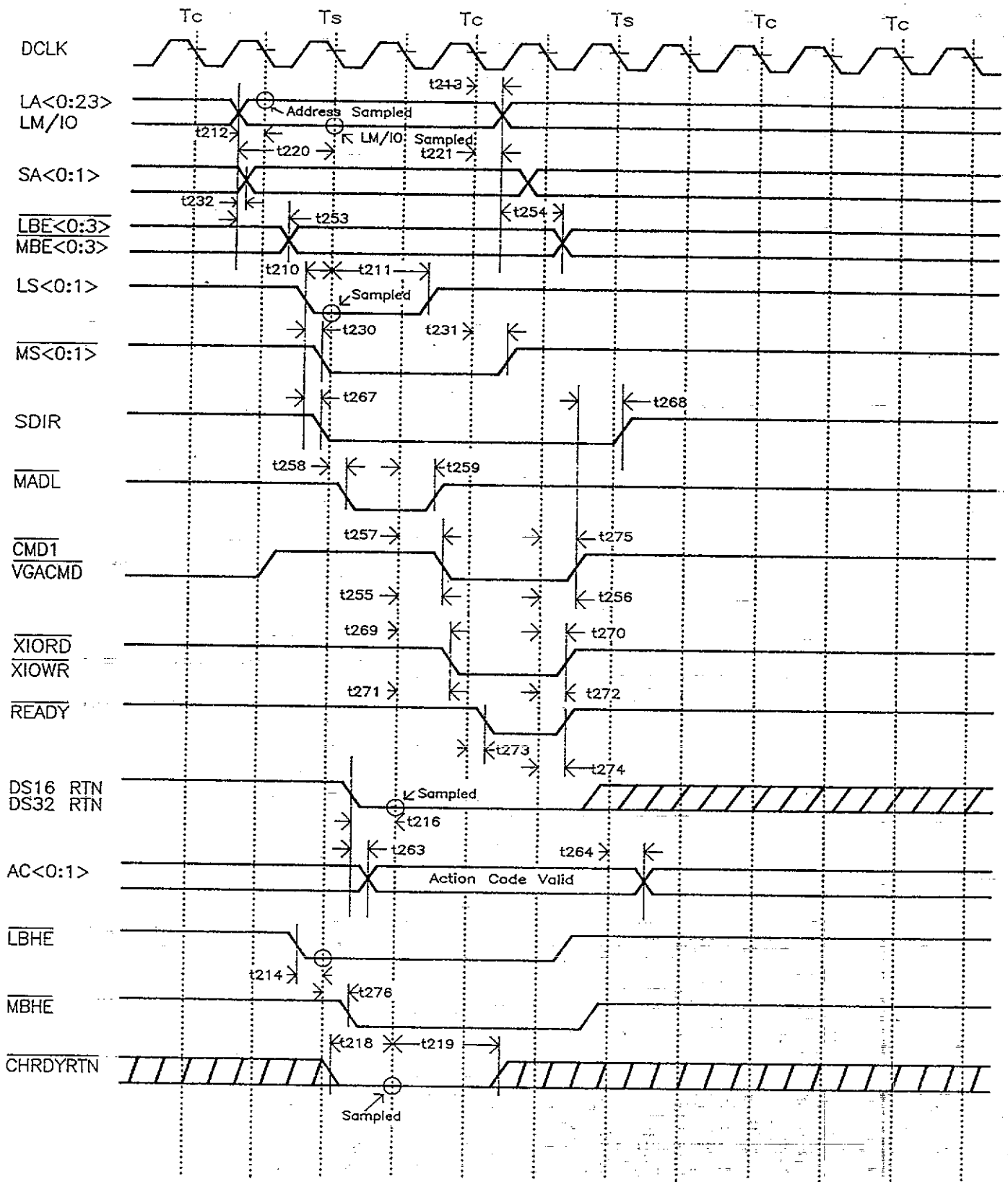
Figure 2.4A 82C321 DMA Cycle (0 Wait State)
