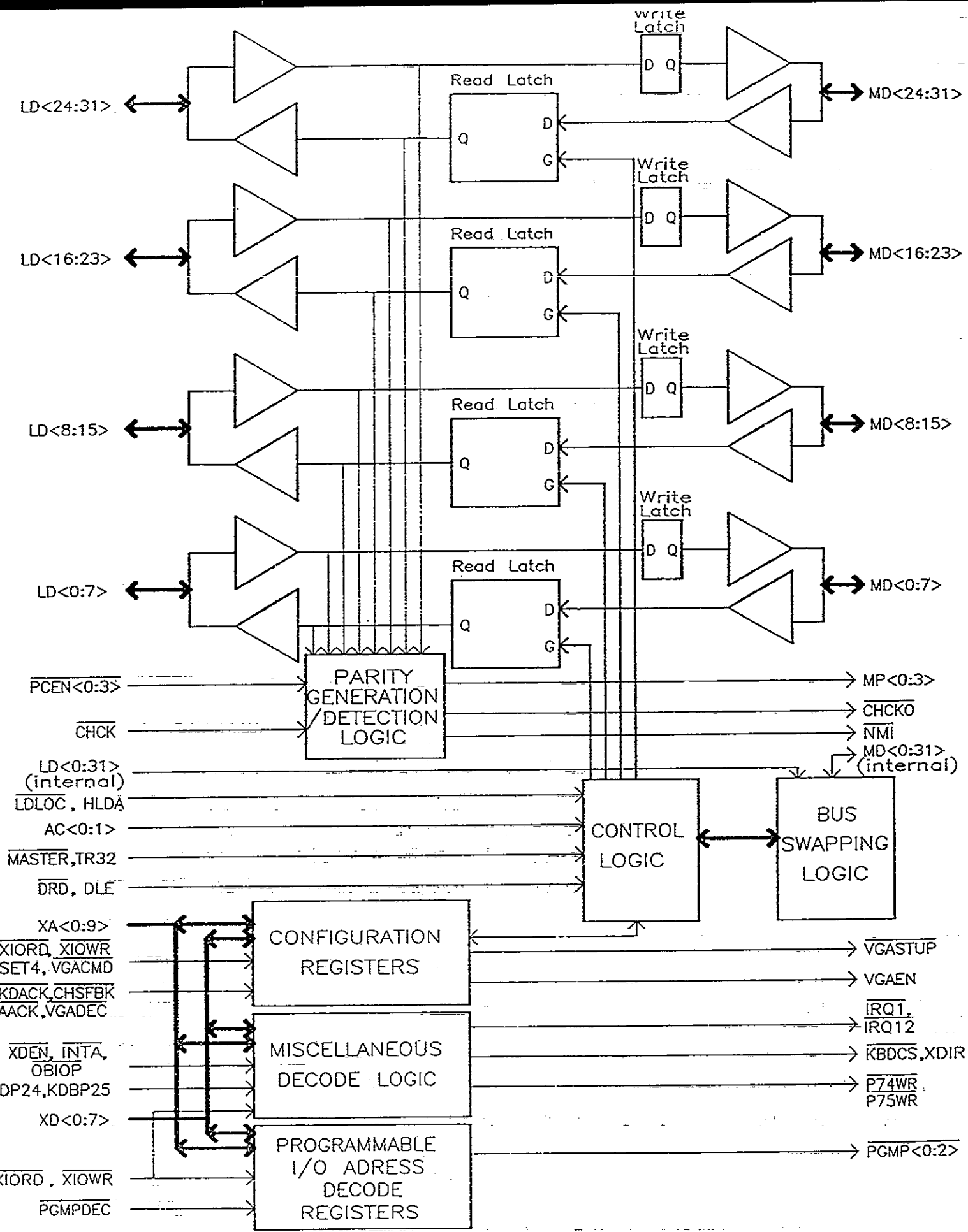
Figure 5.1 82C325 DATA BUFFER Block Diagram
