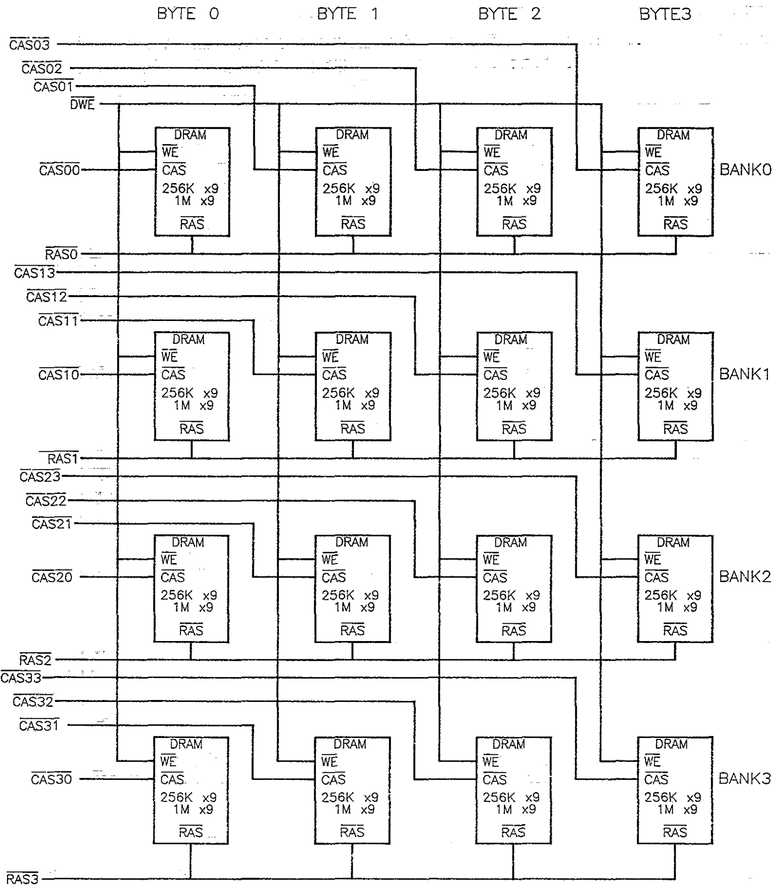
Figure 3.3 DRAM Organization
