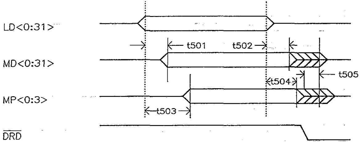
Figure 6.1 CPU Writes to DRAM on MD Bus (DMA Low Word)
