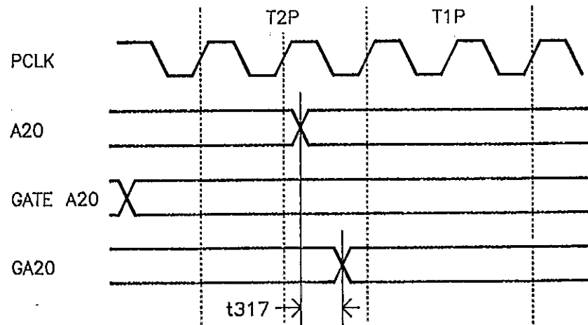
Figure 4.18 GA20 Timing
