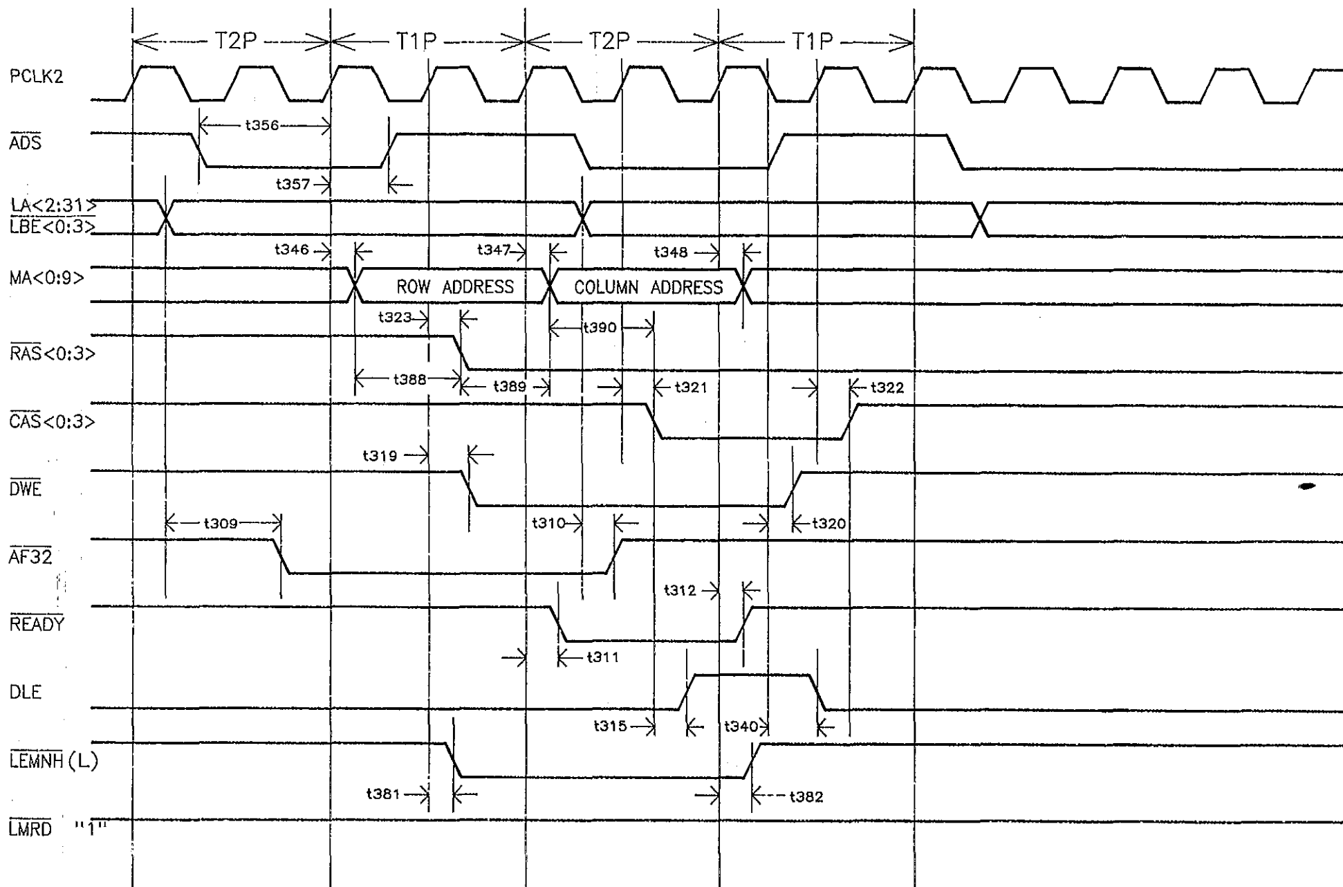
Figure 4.12 Memory on LD Bus, Page Mode, 0 Wait State, RAS High, Write Cycle
