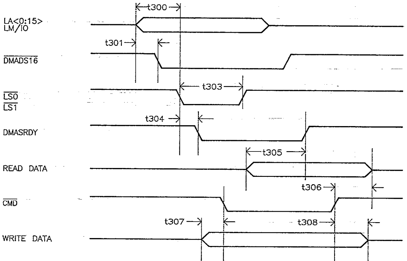
Figure 8.1 SLAVE MODE TIMING
