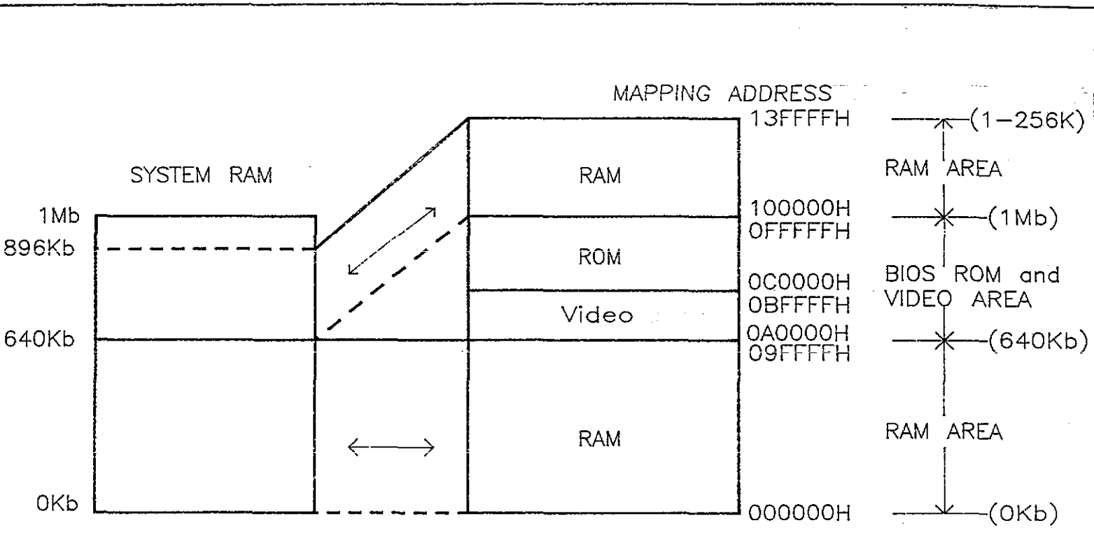
Figure 3.5 System RAM/ROM Mapping for 1MB System RAM
