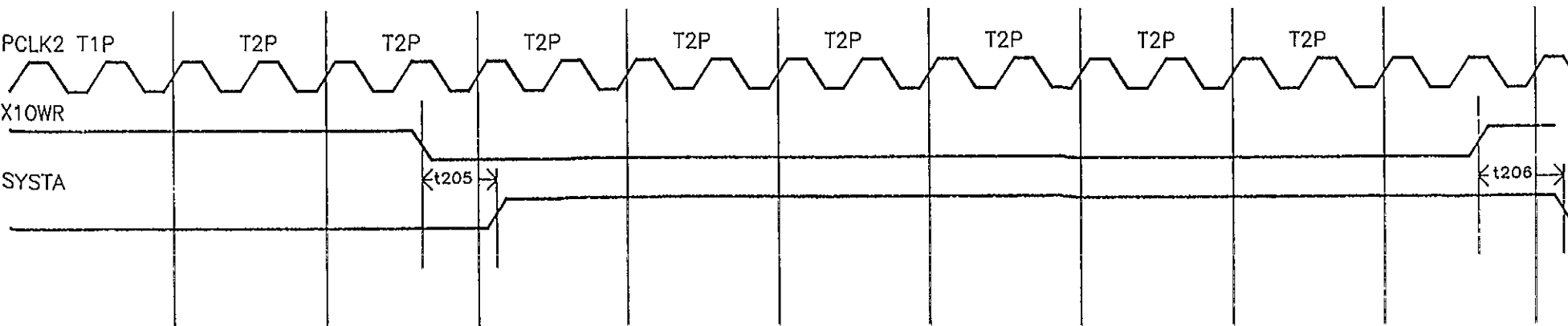
Figure 2.13 SYSTA Timing
