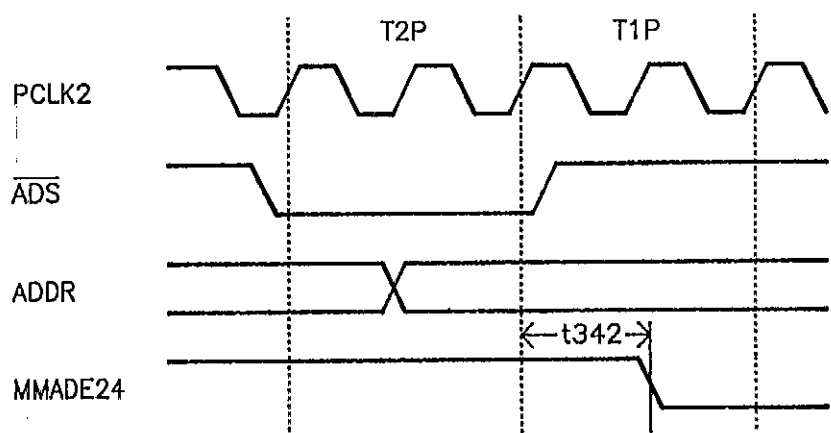
Figure 4.17 MMADE24 Timing
