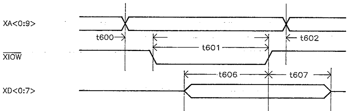
Figure 10.2 226 PERIPHERAL WRITE CYCLE
