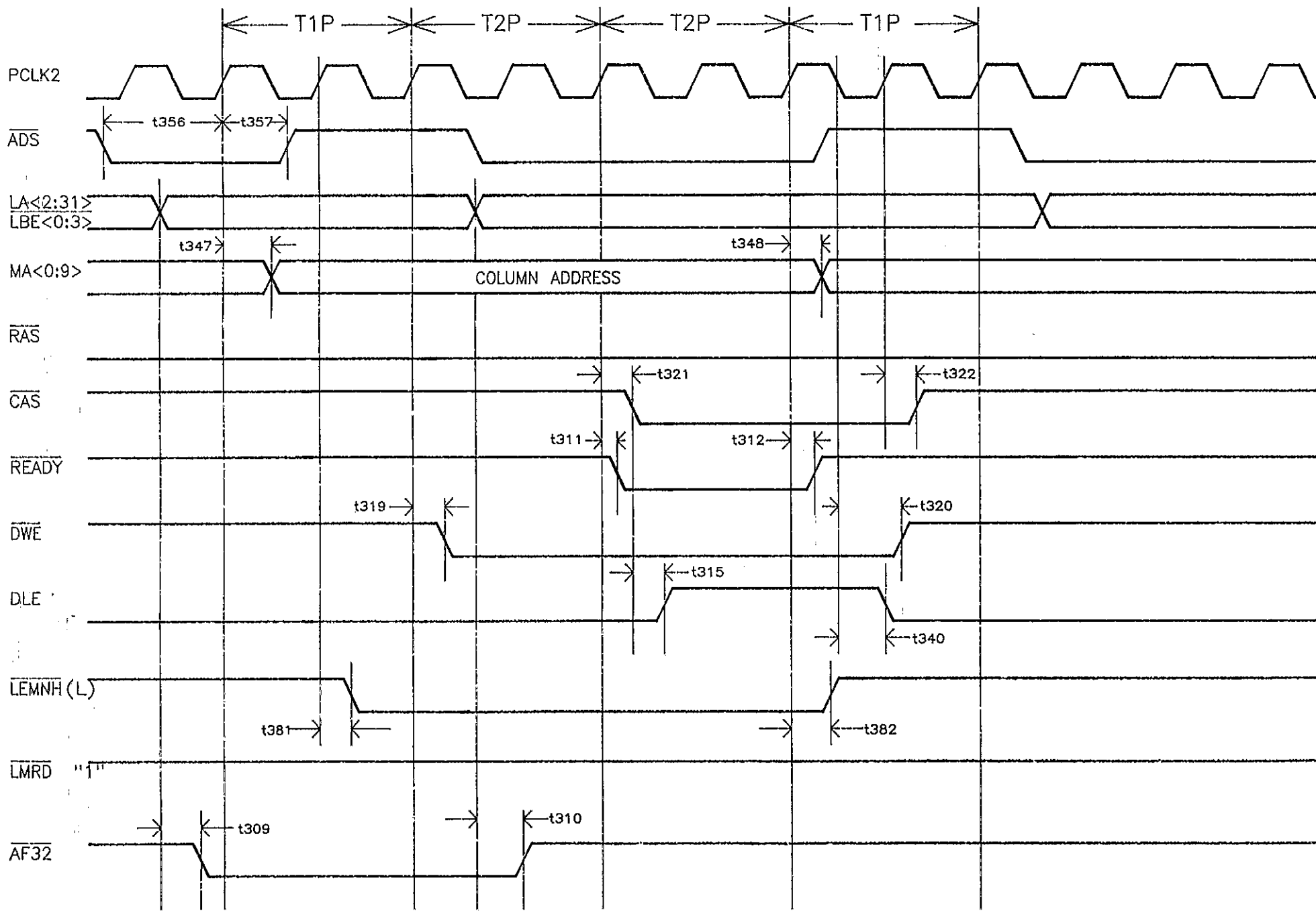
Figure 4.4 Memory on LD Bus, Page Mode, 1 Wait State, Write Hit Cycle
