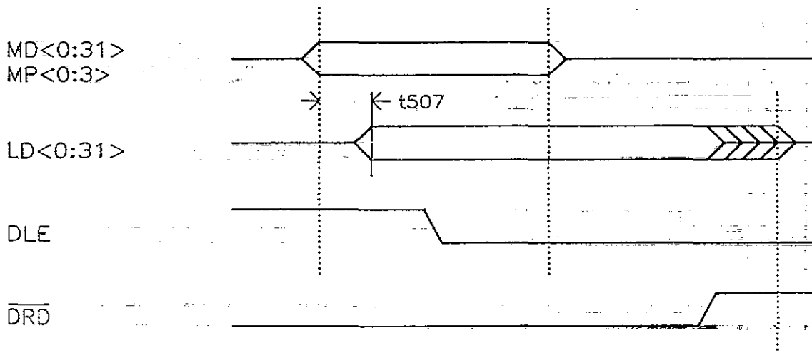
Figure 6.2 CPU Reads DRAM on the MD Bus (DMA Low Word)
