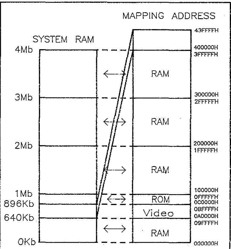
Figure 3.6 RAM/ROM Mapping Without Shadow RAM (More Than 1MB of RAM)
