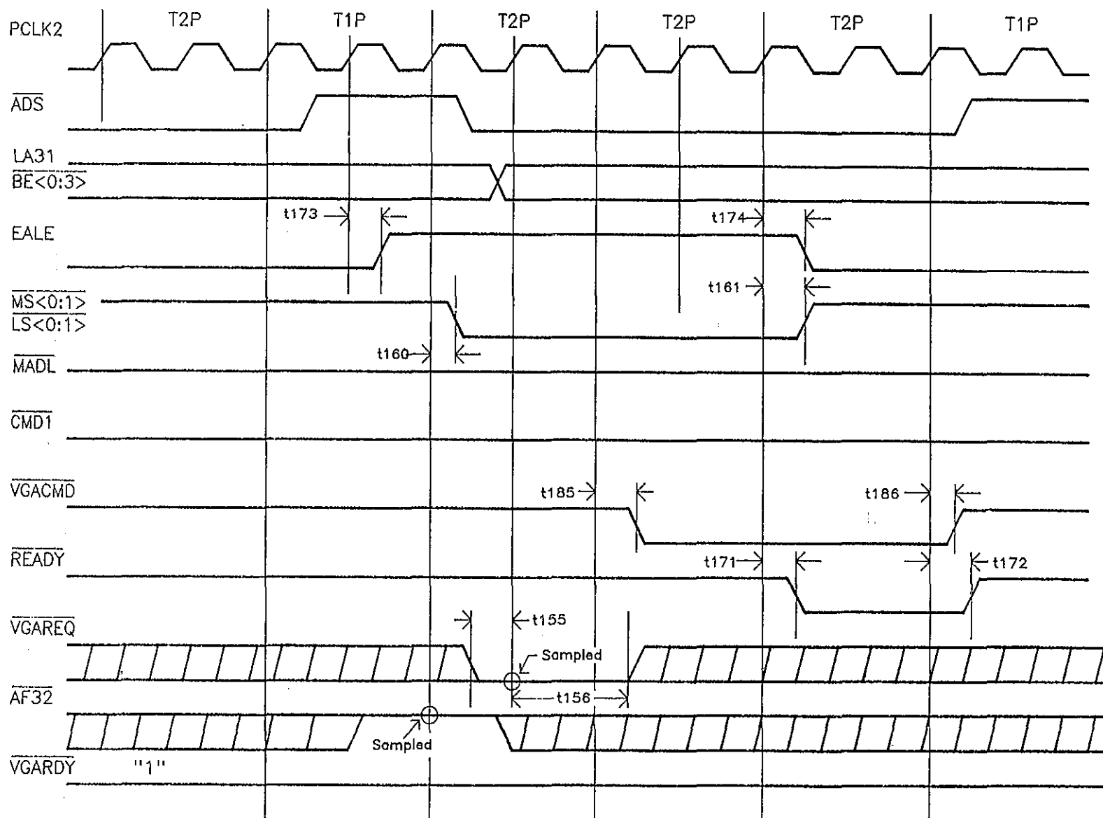
Figure 2.7 20MHz, 25MHz (AF32 Option Enabled) Fast VGA I/O Cycle
