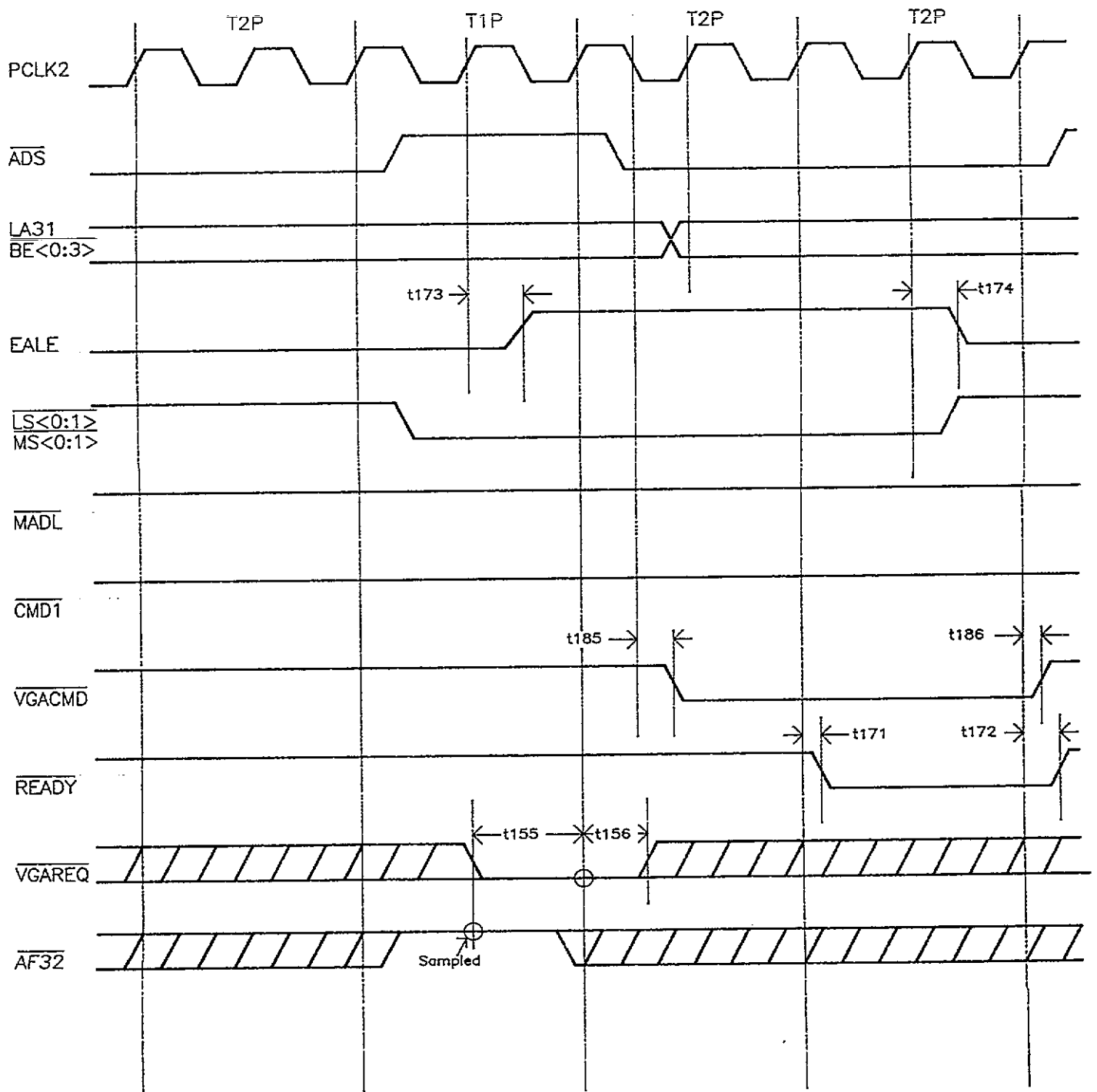
Figure 2.8 16MHz Fast VGA I/O Cycle
