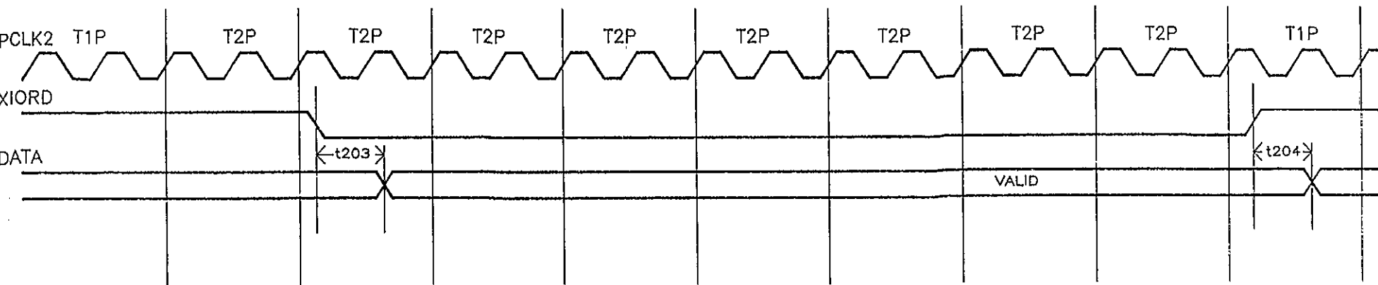
Figure 2.12 Internal Register Access Timing
