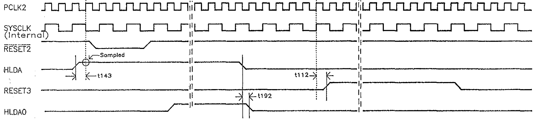
Figure 2.21 RESET2 asserted during HLDA high
