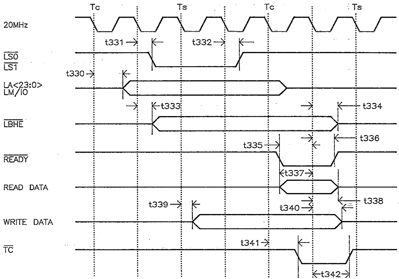
Figure 8.4 MASTER MODE
