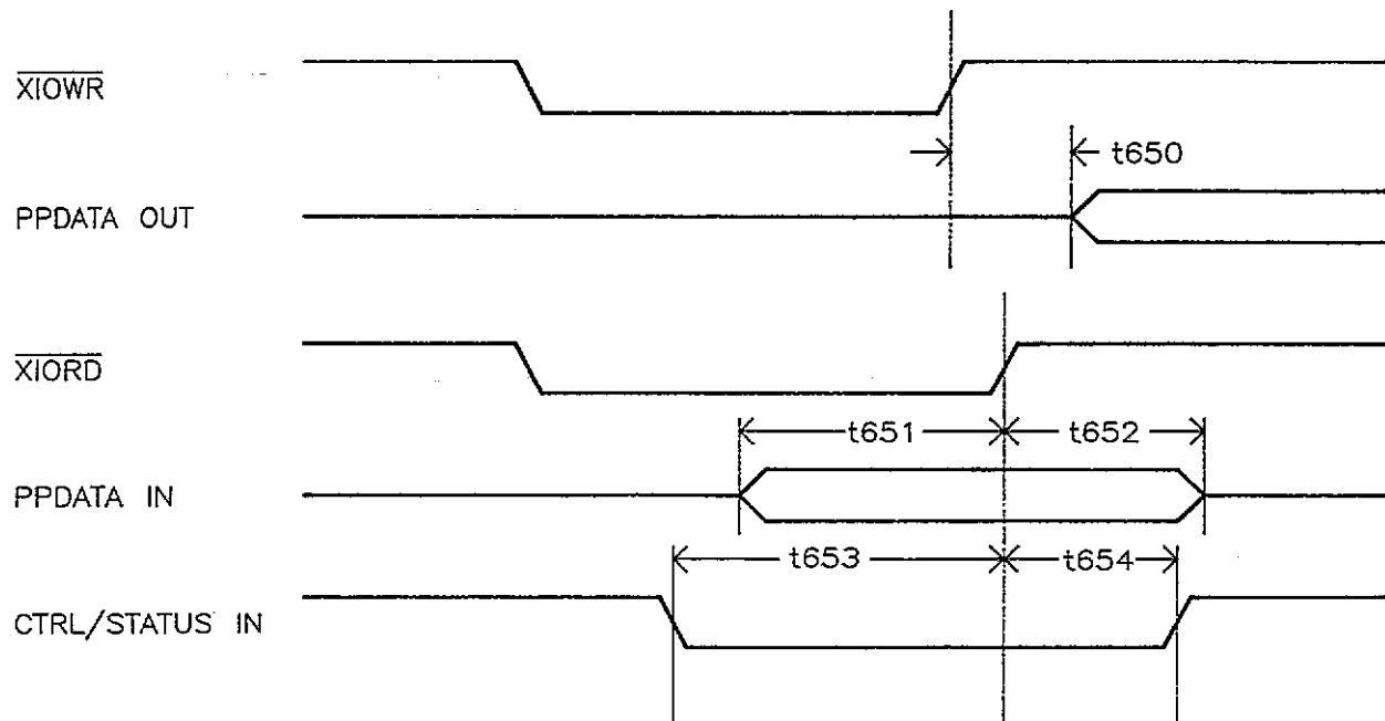
Figure 10.3 PARALLEL PORT
