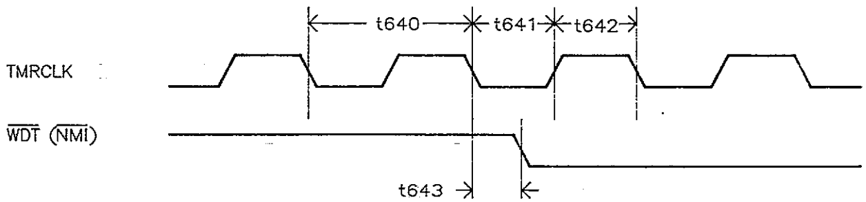
Figure 10.8 WATCHDOG TIMER
