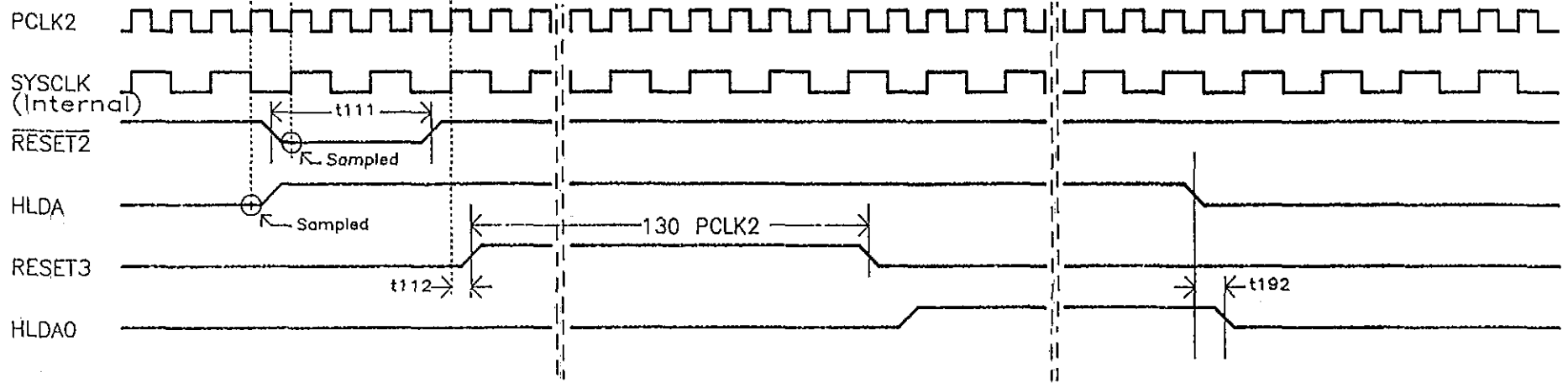
Figure 2.20 RESET2 and HLDA asserted simultaneously
