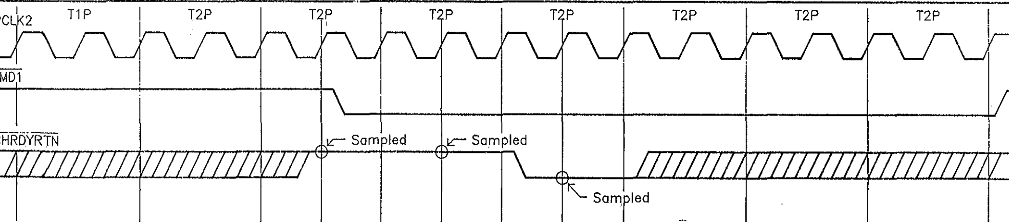
Figure 2.23 25 MHz Asynchronous Extended Cycle
