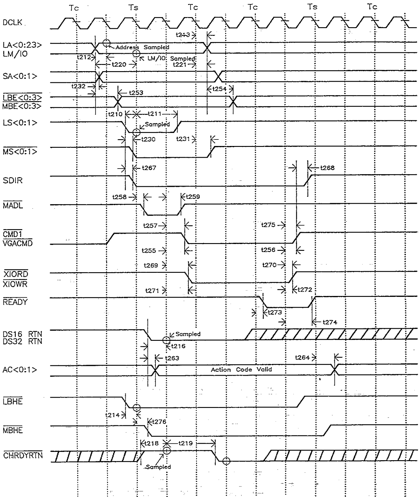
Figure 2.4 82C321 DMA Cycle (1 Wait State)
