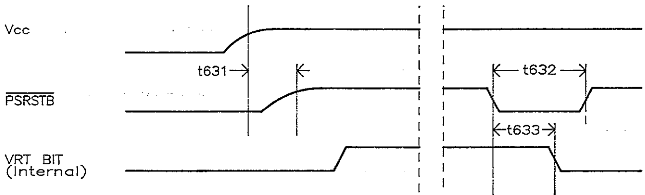
Figure 10.7 226 REAL TIME CLOCK POWER-UP SEQUENCE
