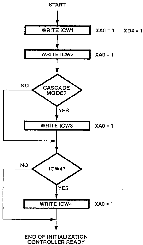
FIGURE 9-6 INITIALIZATION SEQUENCE
