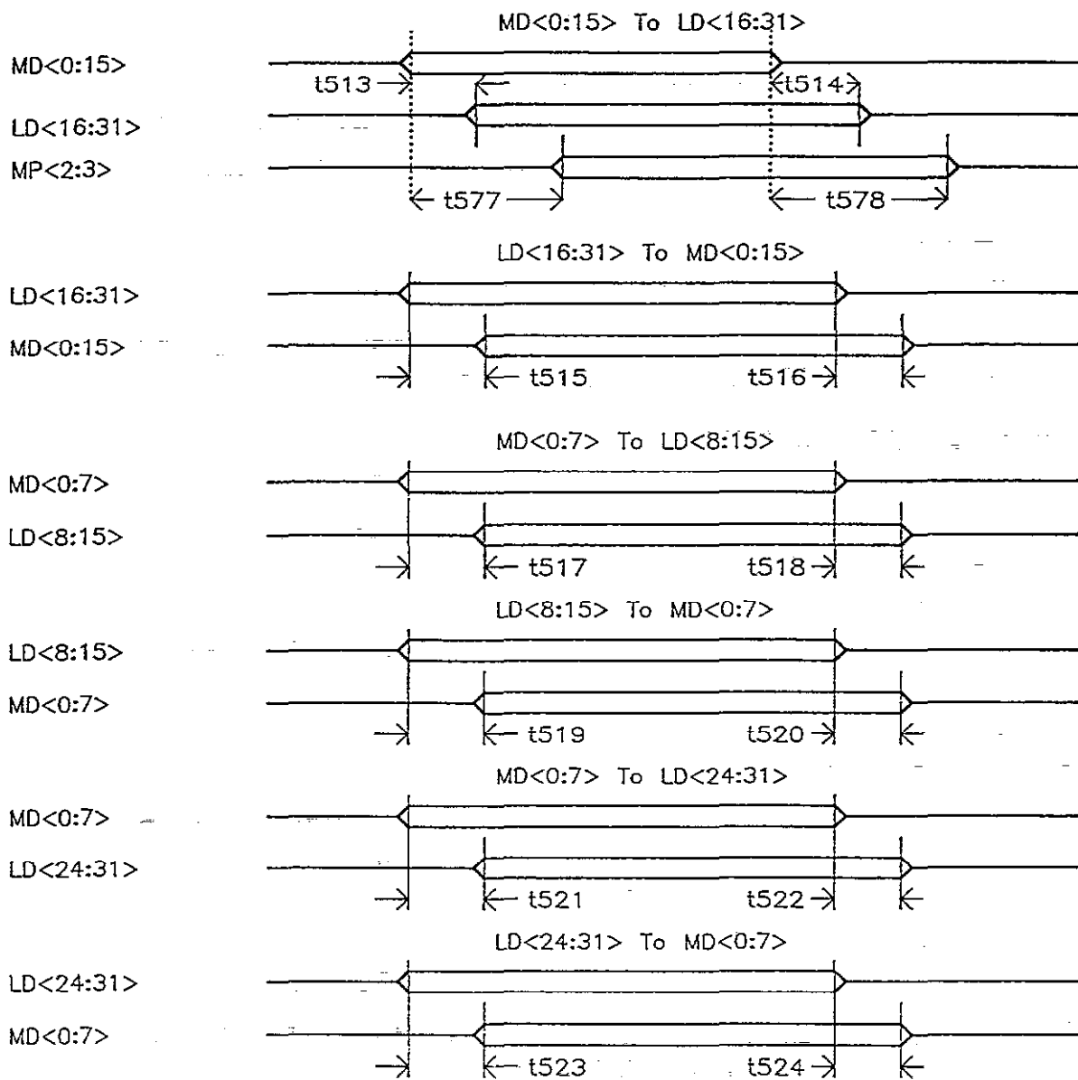
Figure 6.3 Path Propagation Delays
