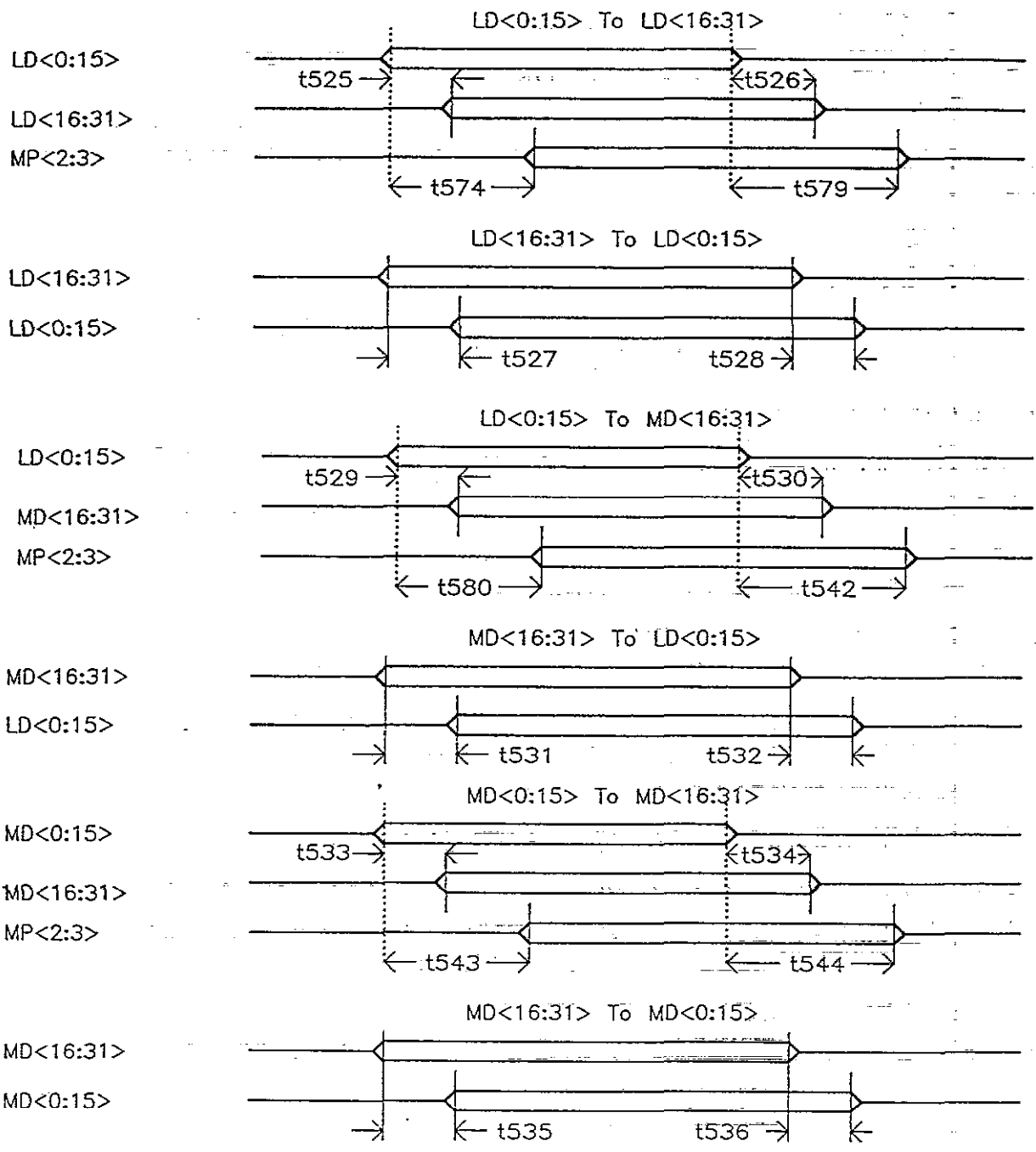
Figure 6.4 Path Propagation Delays
