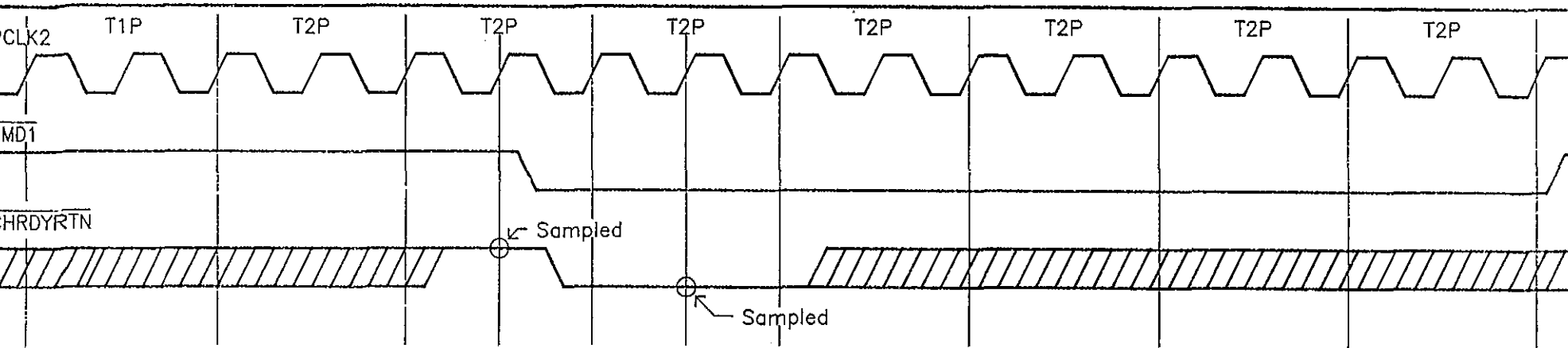
Figure 2.22 25 MHz Synchronous Extended Cycle
