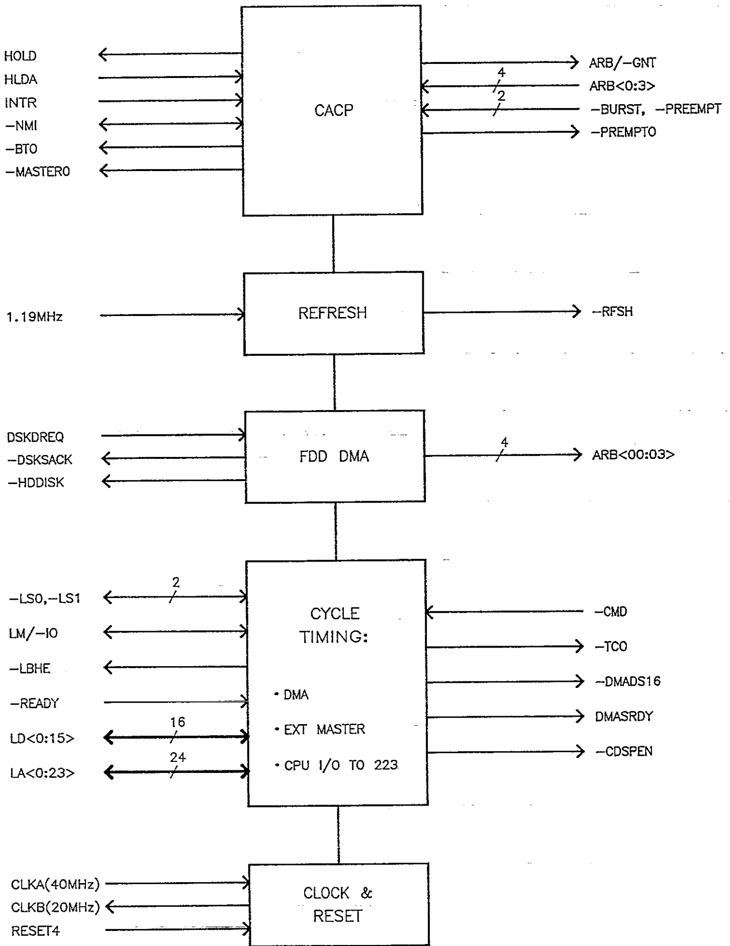
Figure 7.1 82C223 Block Diagram
