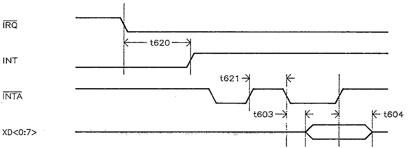
Figure 10.6 INTA SEQUENCE
