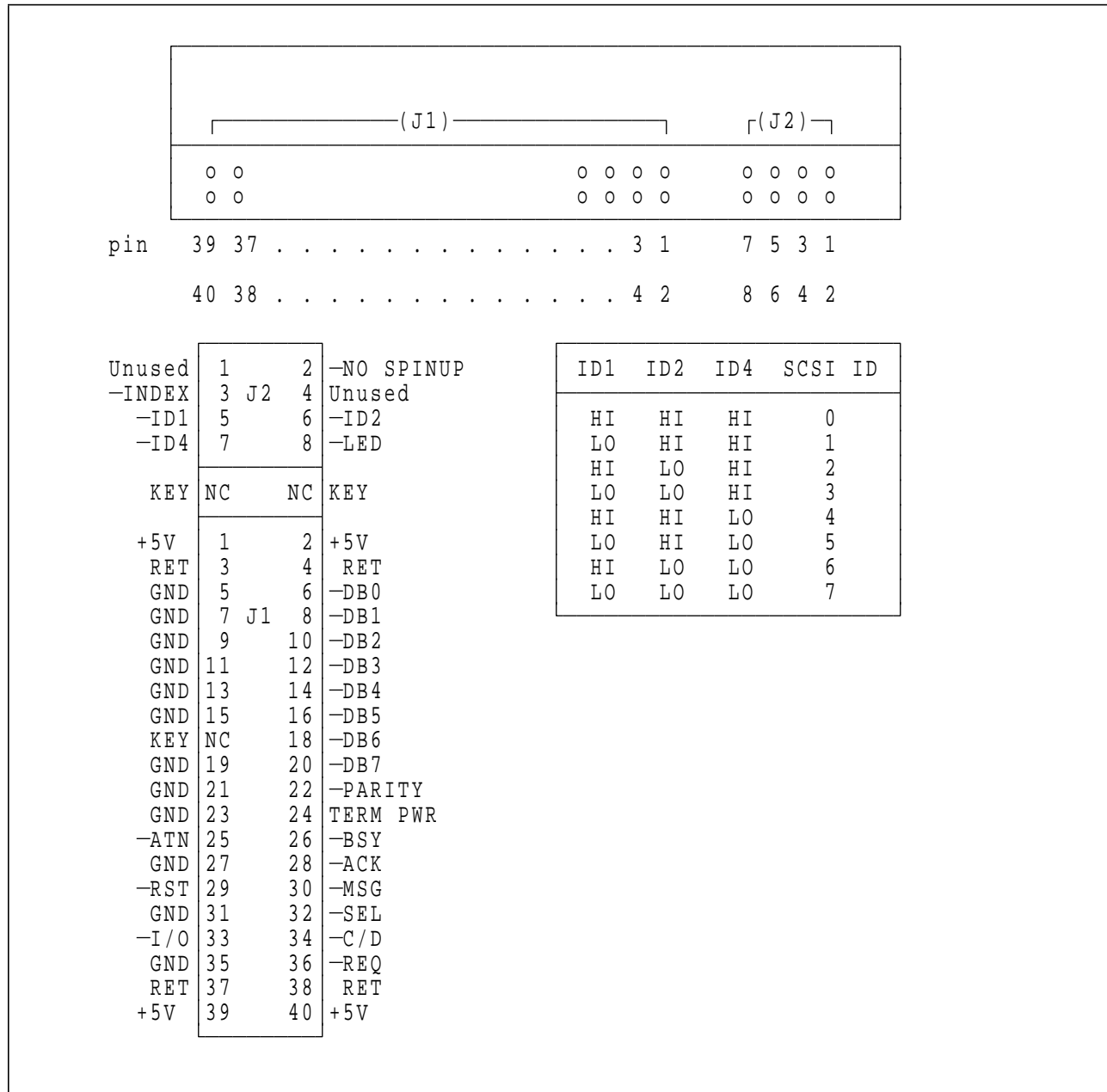
Figure 5-2. 40 pin SCSI Connector
