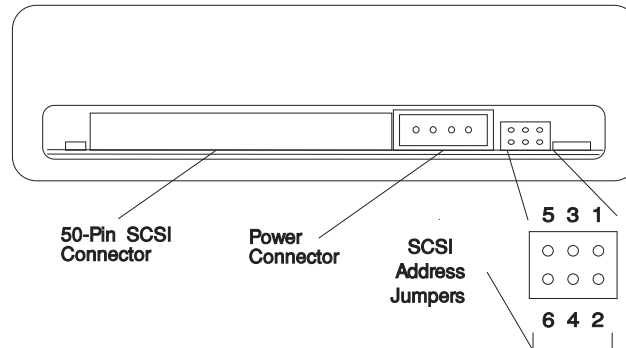
8-mm Tape (Back View)
