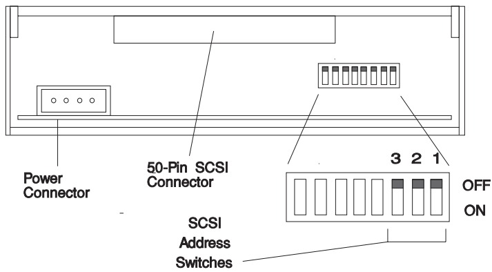
4 mm Tape (Back View)
