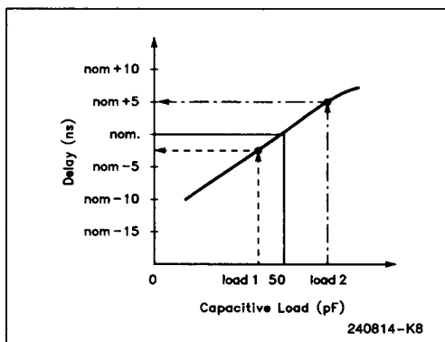
Using the Capacitive Derating Curves
