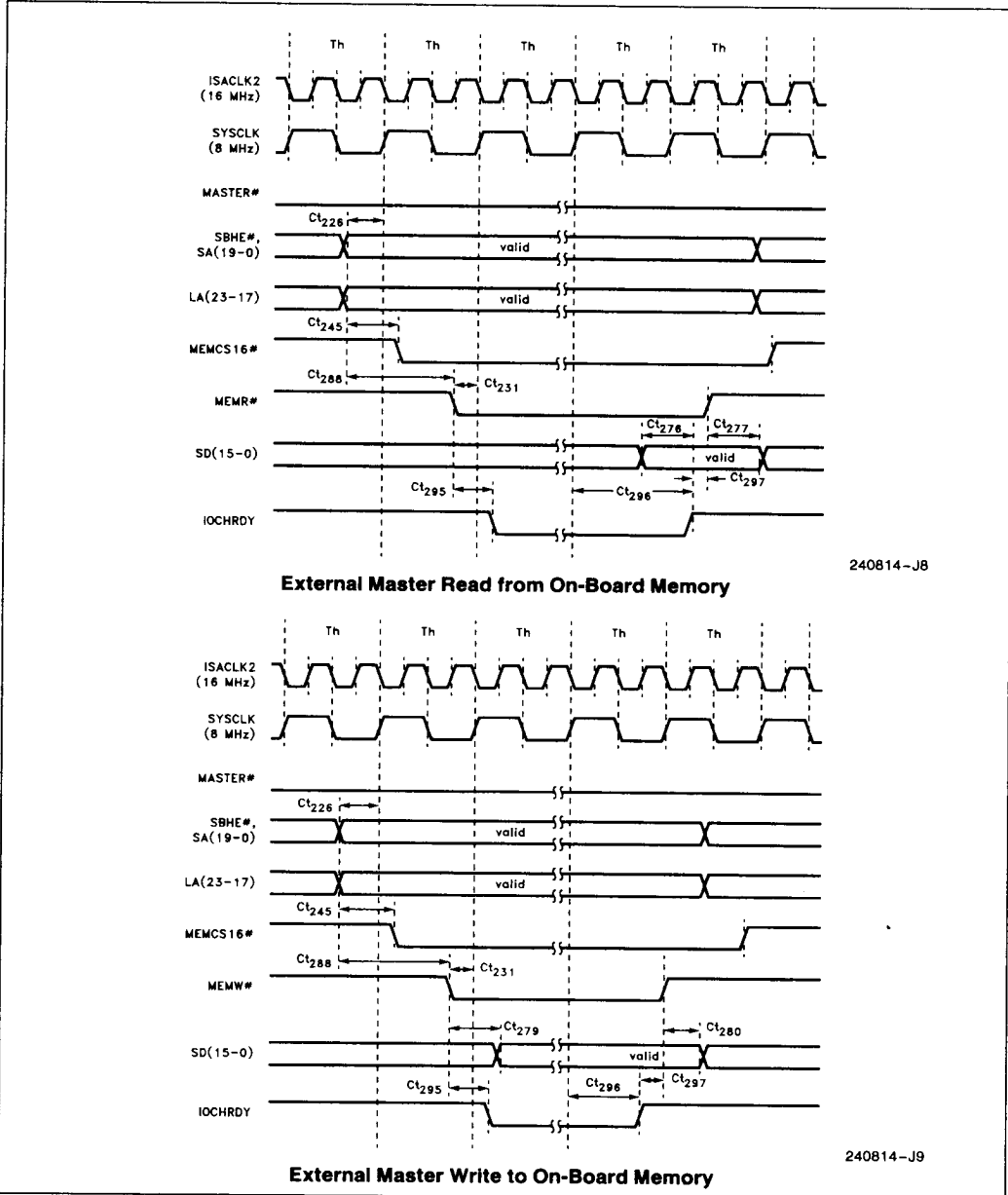
Figure 3.5.28b. ISA Bus External Bus Master Accesses to On-Board Memory
