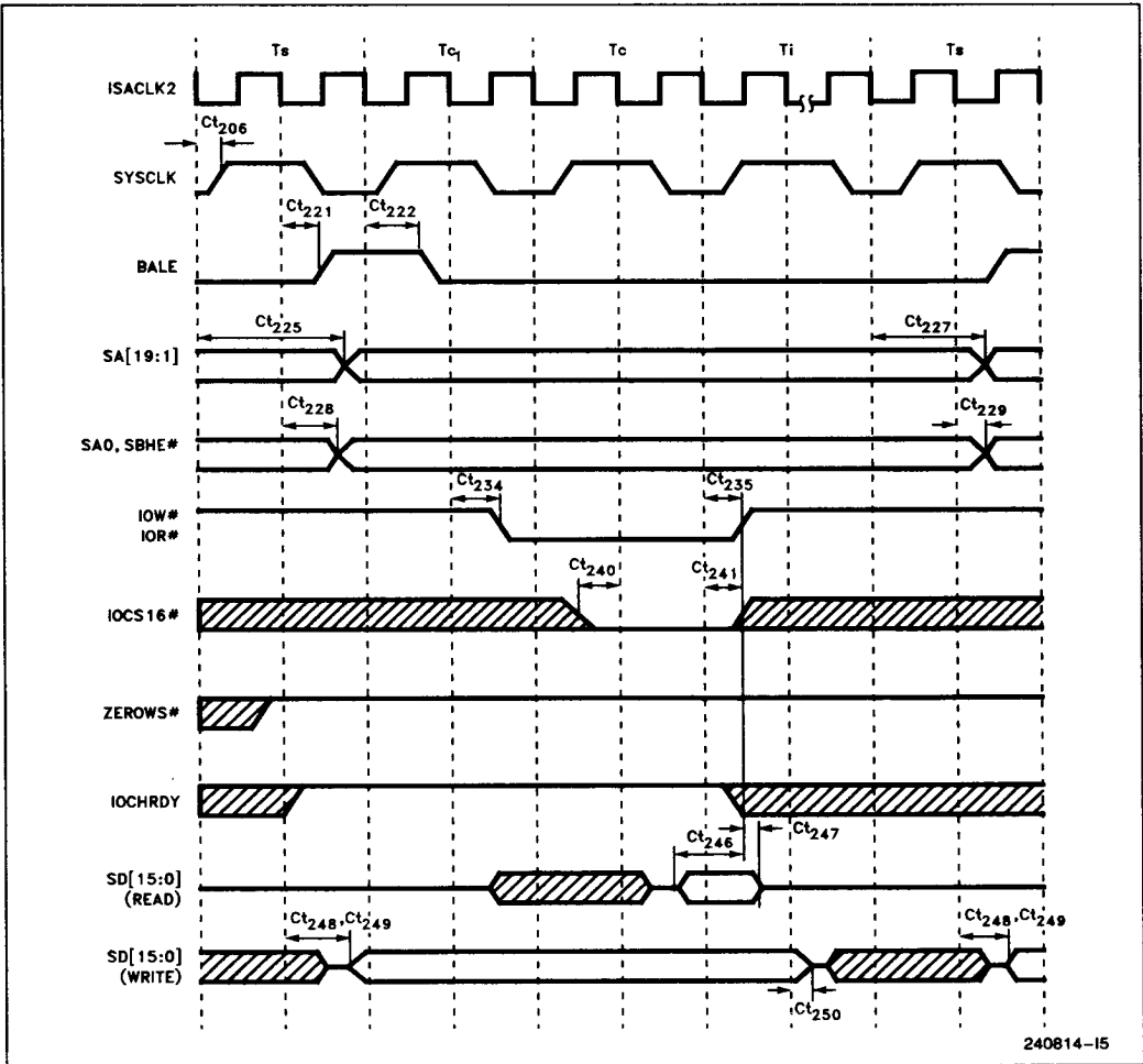
Figure 3.5.21. ISA Bus 16-Bit I/O Read/Write Standard ISA Bus Cycles (3 SYSLKs)
