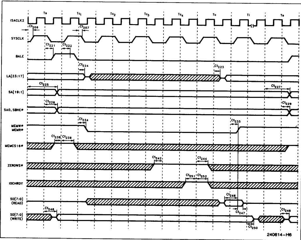
Figure 3.5.12. ISA Bus 8-Bit Memory Read/Write Standard ISA Bus Cycle (6 SYSCALLs)
