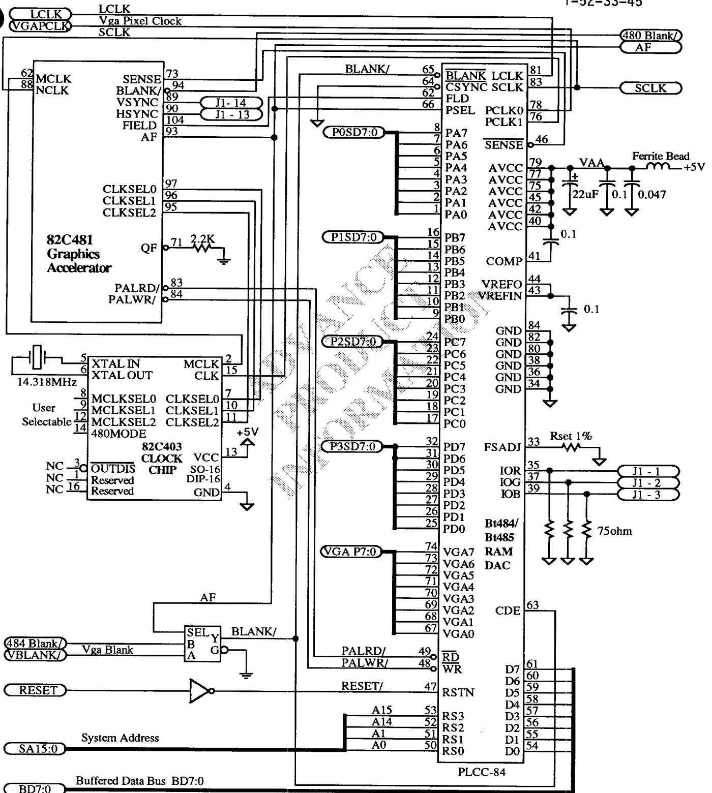
82C481 Video Circuit Example - High Performance RAMDAC (BT484 / 485)
