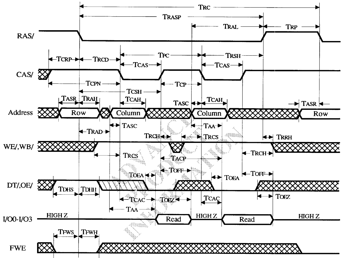
VRAM Fast-page Read Cycle Timing
