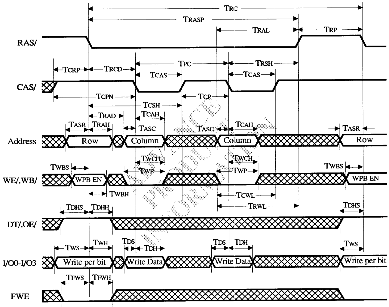
VRAM Fast-page Write Cycle Timing
