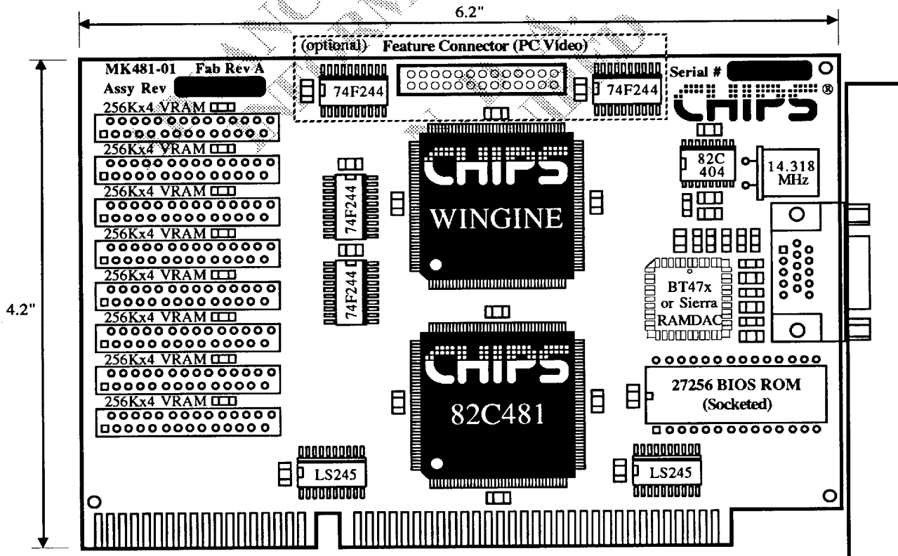
Example Wingine / 82C481 PCB
