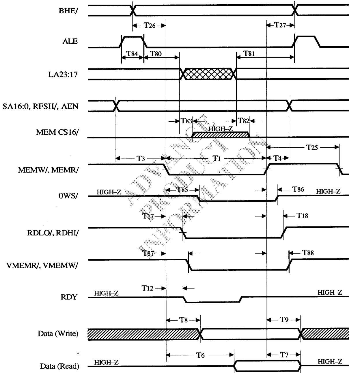
UISA Bus 16-Bit Memory Cycle Timing
