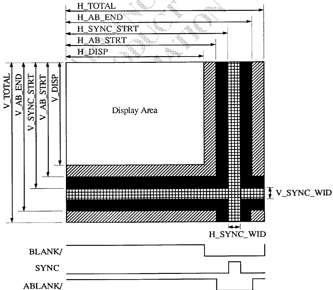
82C481 Video Timing Signals
