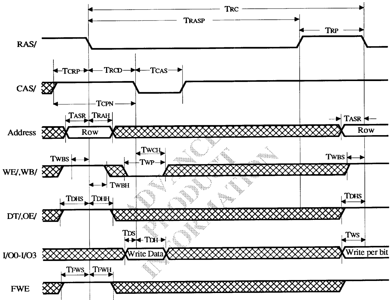
VRAM Color Register Set Cycle Timing
