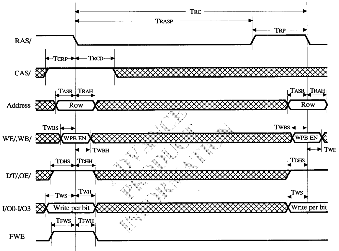
VRAM Flash Write Cycle Timing
