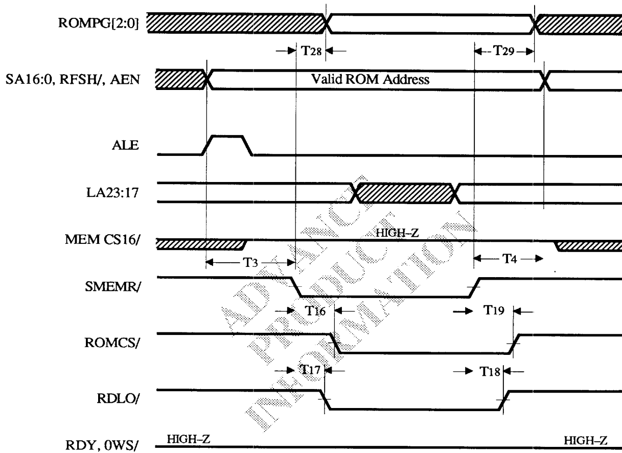
UISA Bus ROM Memory Cycle Timing
