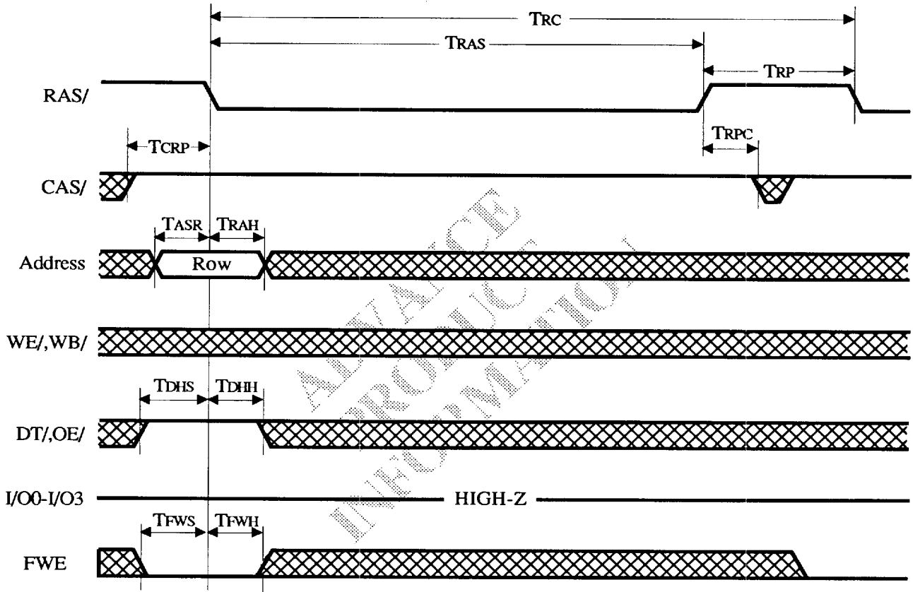
VRAM Refresh Cycle Timing
