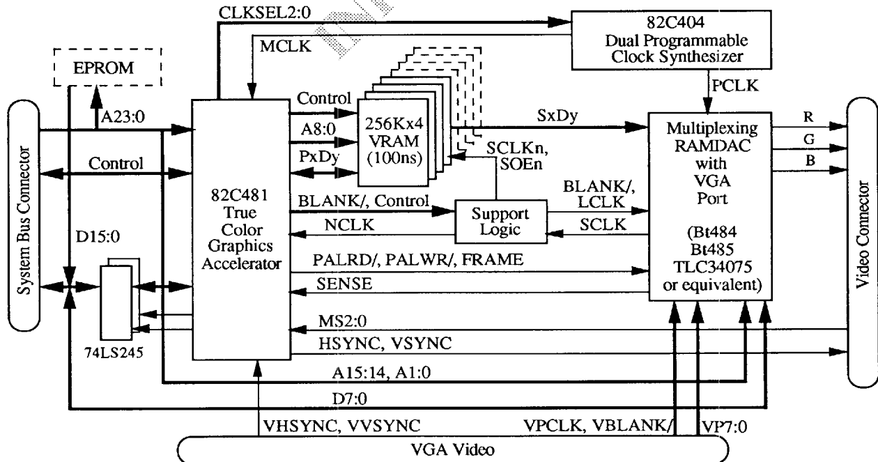
82C481 System Block Diagram
