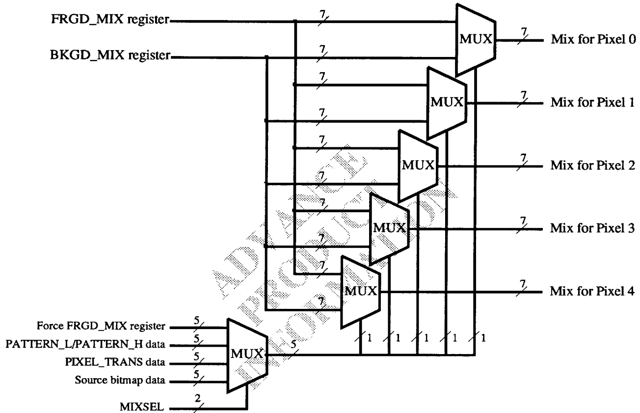
Mix Select for each Pixel Drawing Engine
