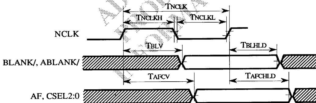
82C481 Nugget Clock Timing
