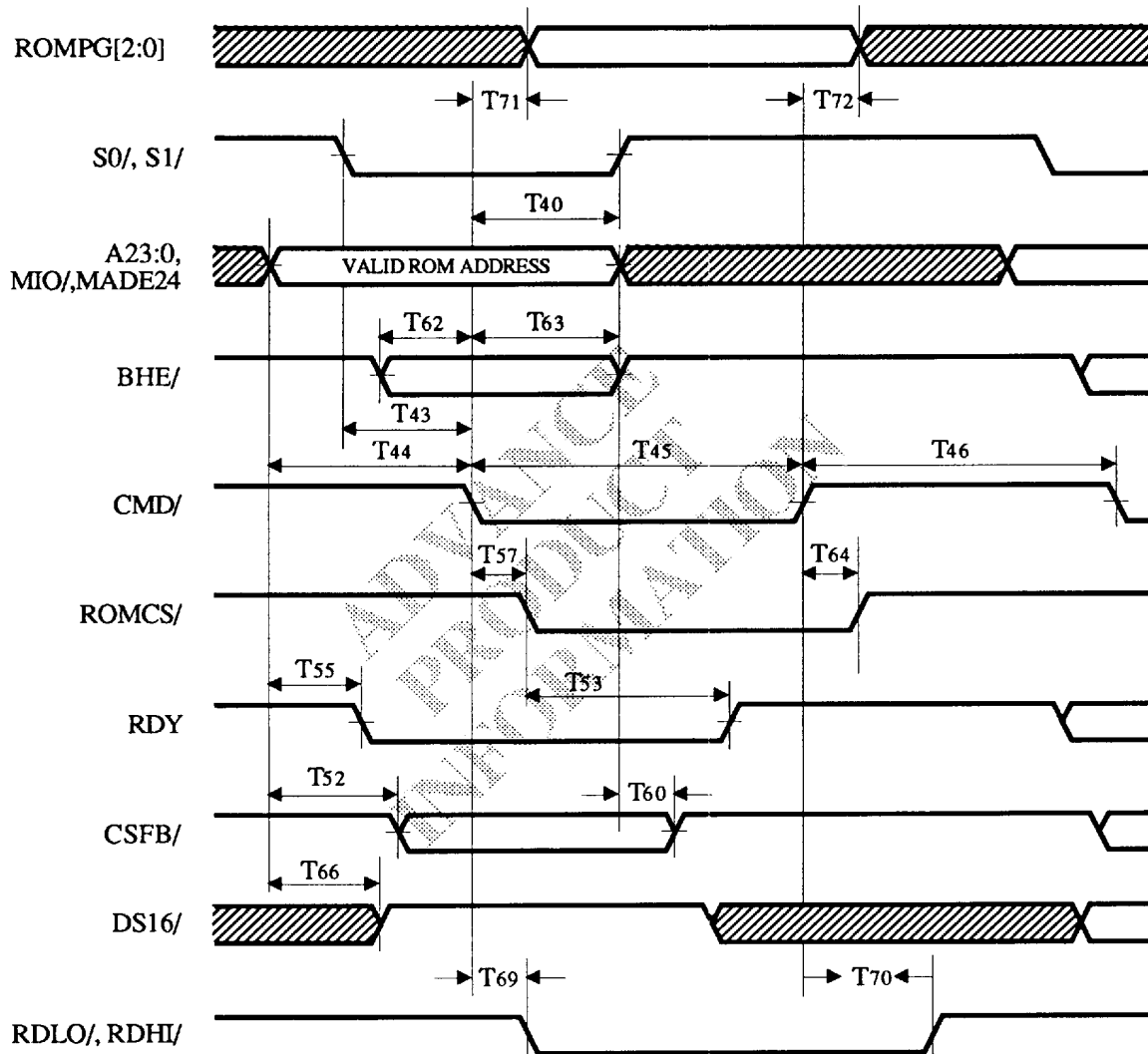
Micro Channel Bus ROM Memory Cycle Timing
