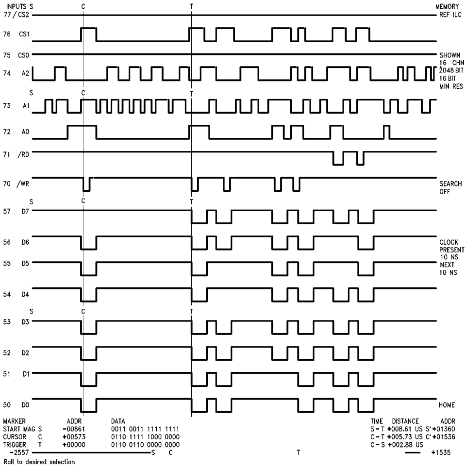
PS/2 Model 50 and 80 Dual ASYNC card initialization for COM2. The cursor shows the second write to the UART. The first write is shown on the "Back-TO-Back write to SCR Read from SCR" Timing Diagram
