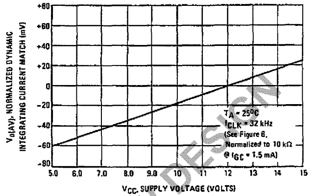
FIGURE 8 - NORMALIZED DYNAMIC INTEGRATING CURRENT MATCH versus V_{CC}
