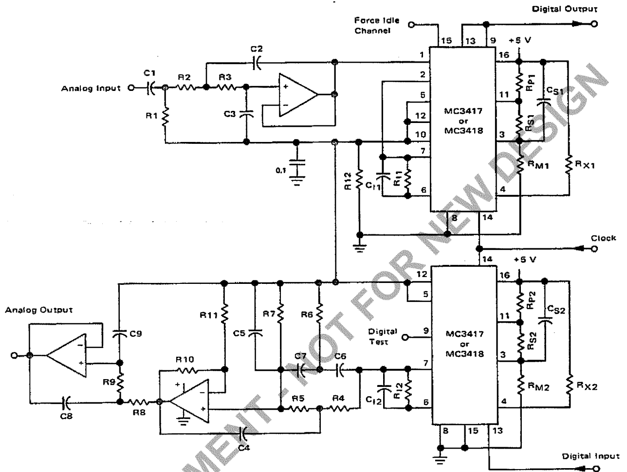
FIGURE 21 — FULL DUPLEX/32K BIT CVSD VOICE CODEC USING MC3517/18 AND MC3503/6 OP AMP
