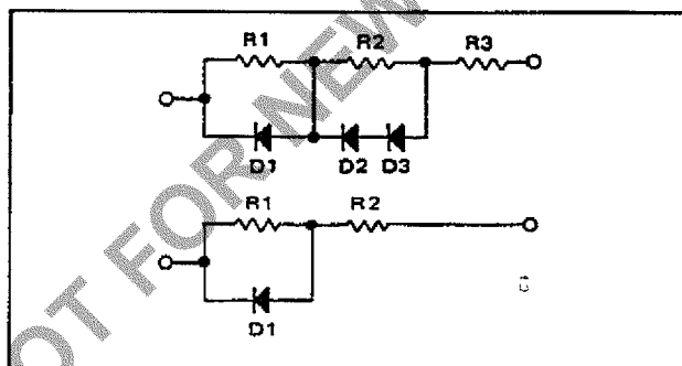
FIGURE 17 - RESISTOR-DIODE NETWORKS
