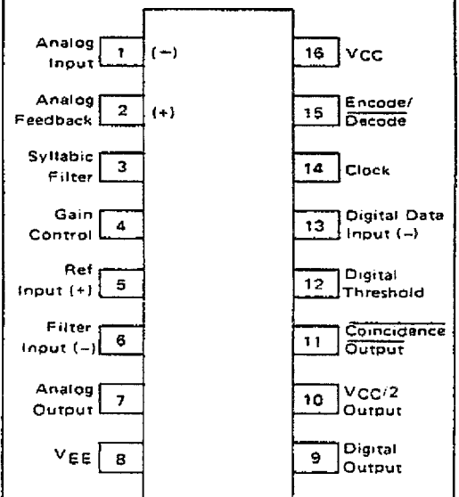
PIN CONNECTIONS
