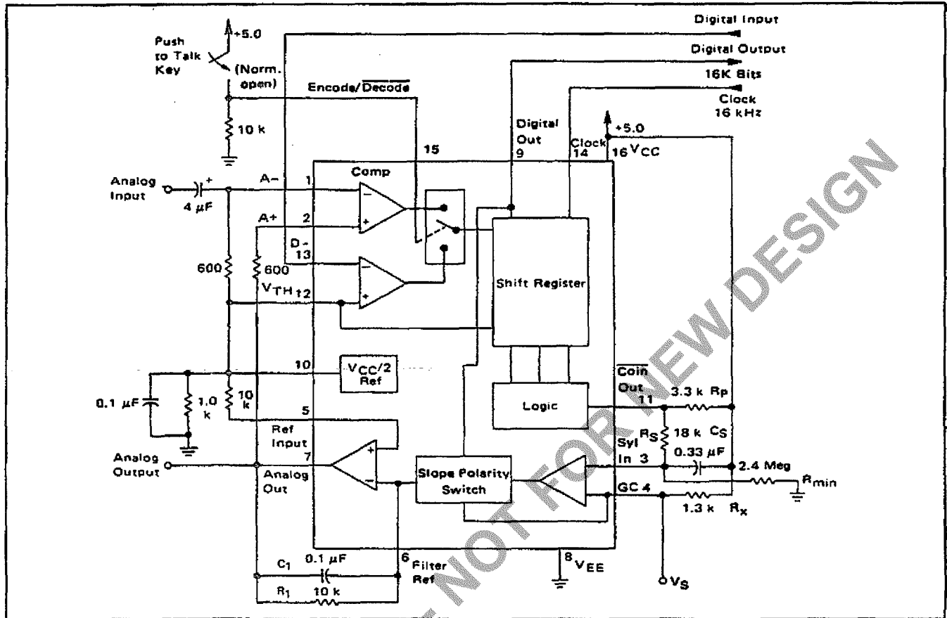
FIGURE 14 – 16 kHz SIMPLEX VOICE CODEC (Using MC3417, Single Pole Companding and Single Integration)
