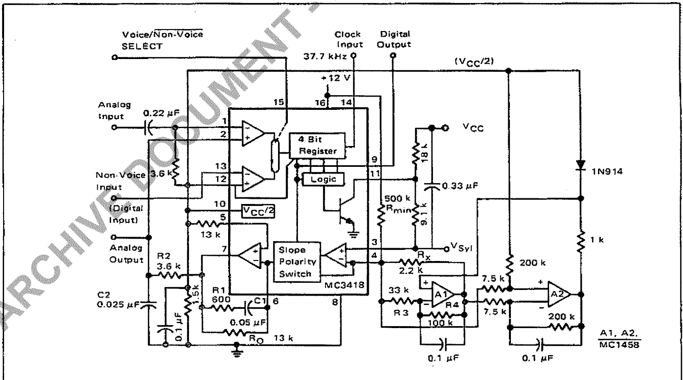
FIGURE 18 - TELEPHONE QUALITY DELTAMOD CODER
