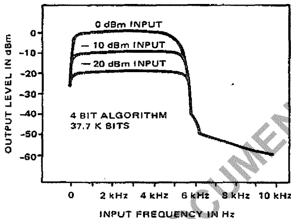
FIGURE 20 – HIGH PERFORMANCE ELLIPTIC FILTER FOR CVSD OUTPUT
