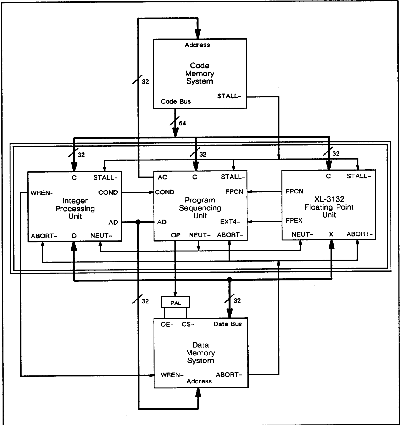
Figure 142. XL-8032 schematic
