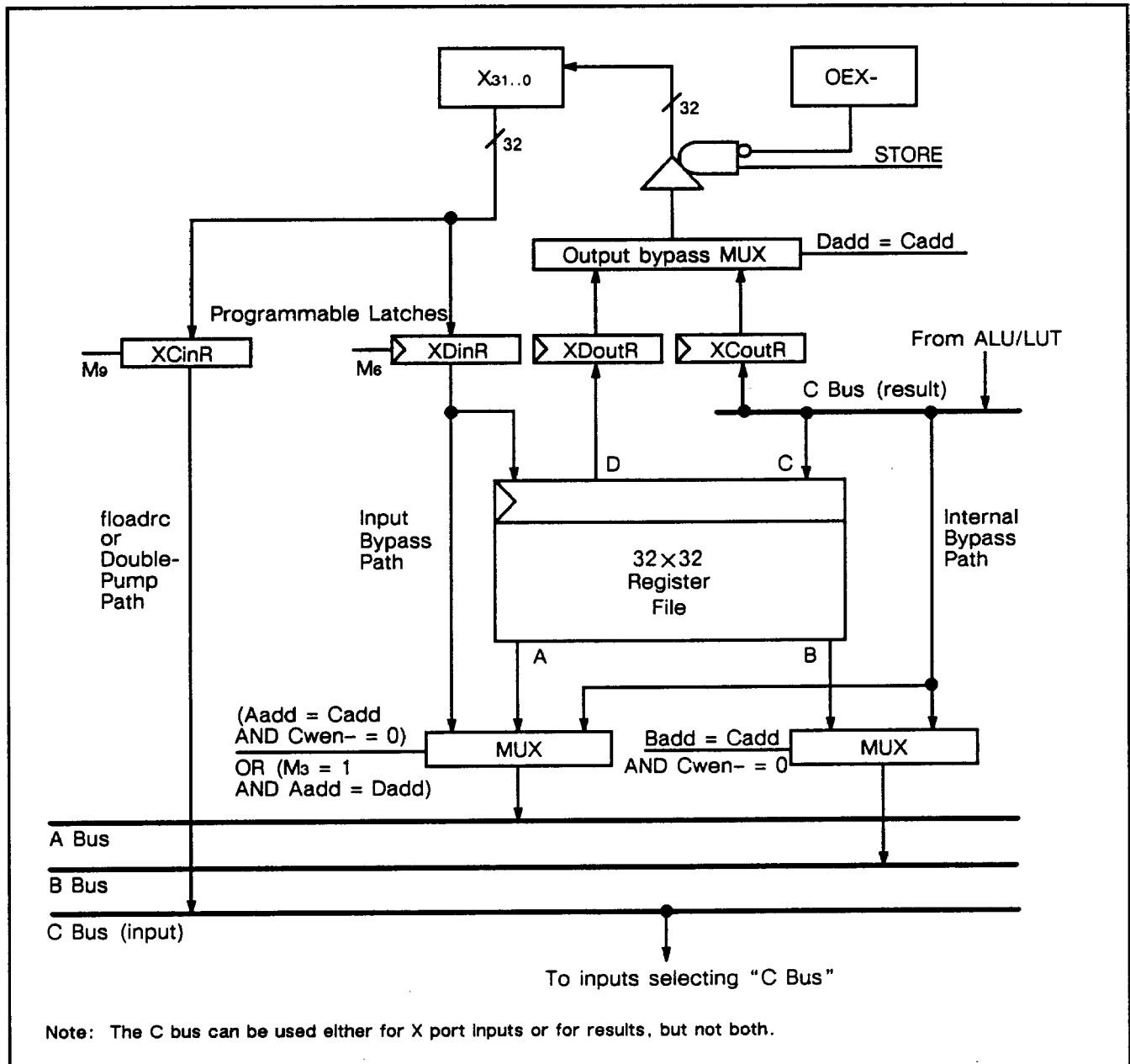
Figure 98. Input/Output Bypass diagram (X port)
