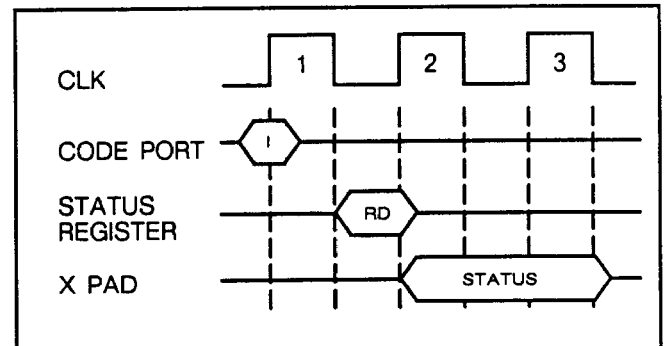
Figure 107. fsts timing
