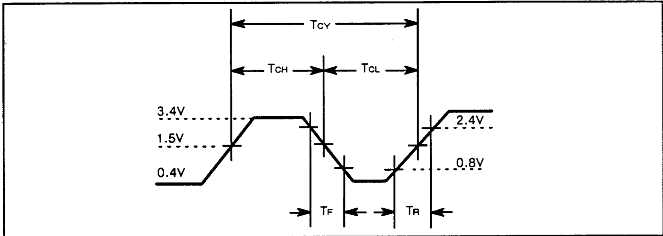
Figure 133. Clock timing
