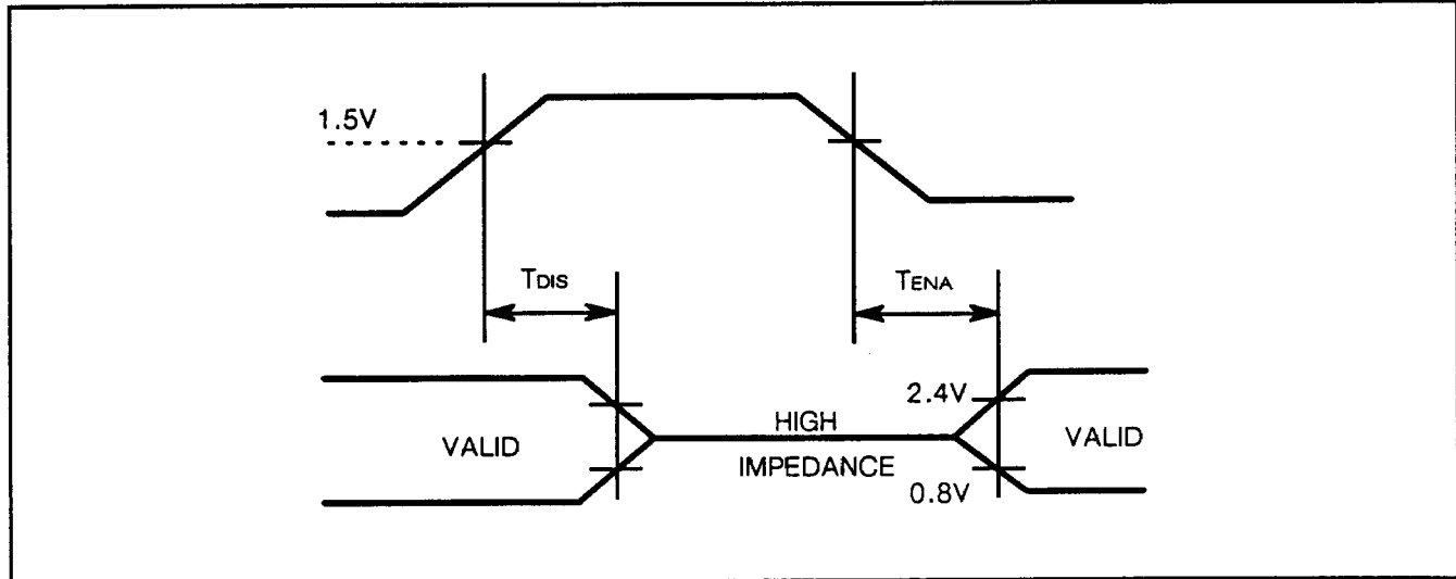
Figure 134. Tri-state timing
