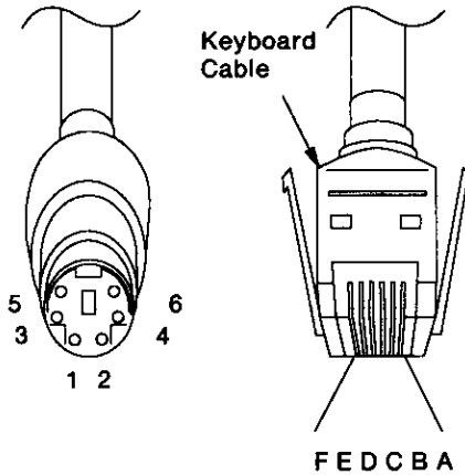
Figure 6-22. Keyboard Cable Connectors
