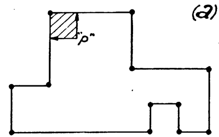
POINT MEMBERSHIP
