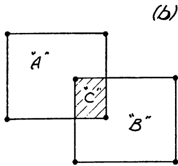
INTERSECTION
