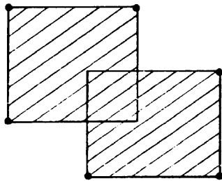
UNION
