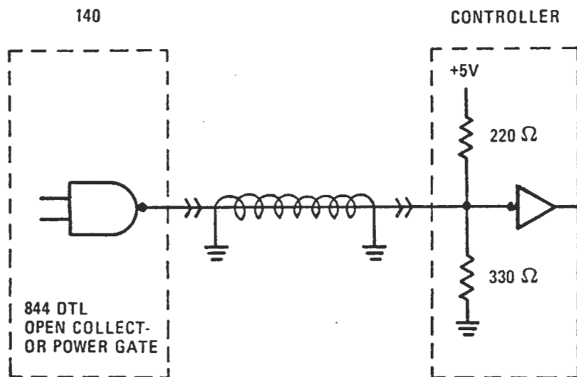
FIGURE 13. DRIVER SCHEMATIC
