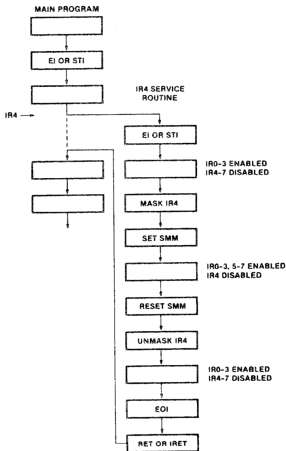
Figure 15. Special Mask Mode Example (MCS 80/85™ or MCS 86/88™)
