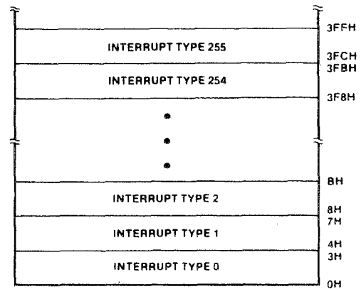
Figure 5. 8086/8088 Interrupt Vector Table
