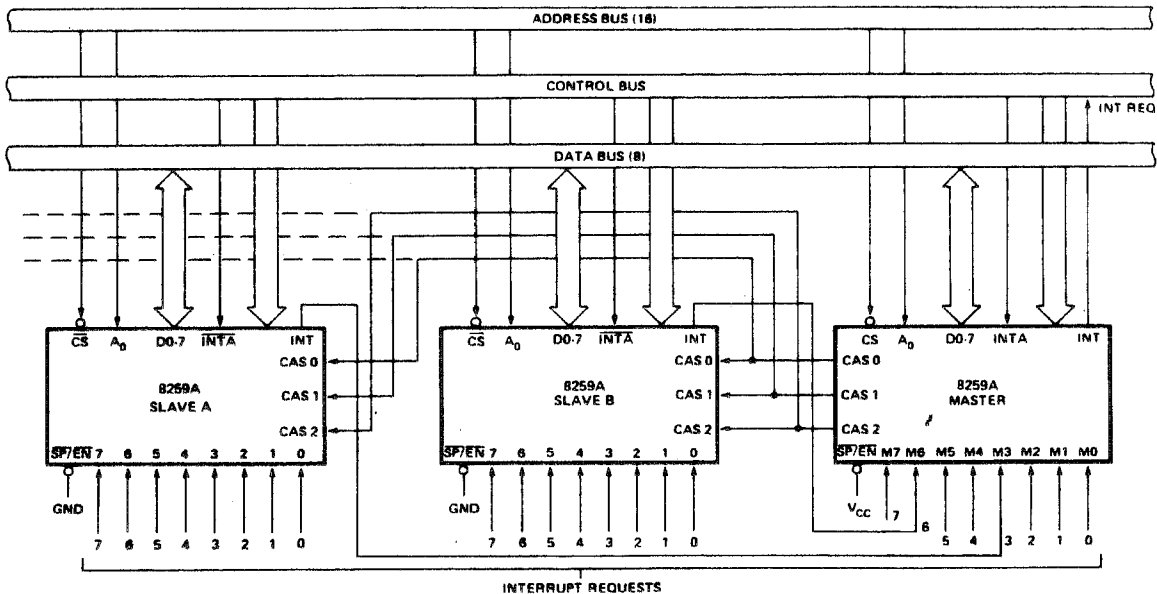
Figure 18. Cascaded 8259A's 22 Interrupt Levels
