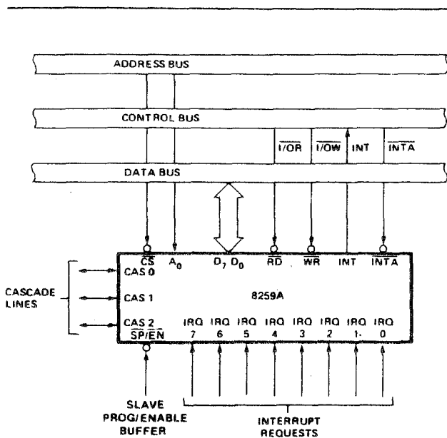
Figure 1. 8259A Interface to Standard System Bus
