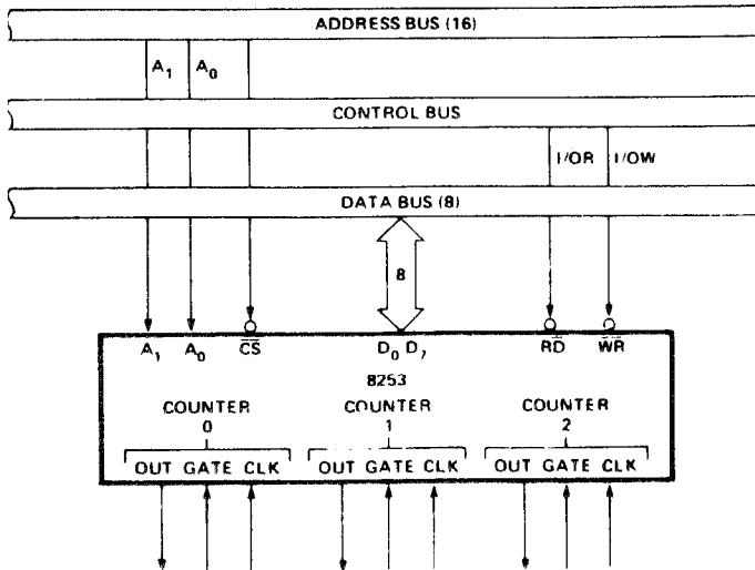
Figure 3. 8253 System Interface
