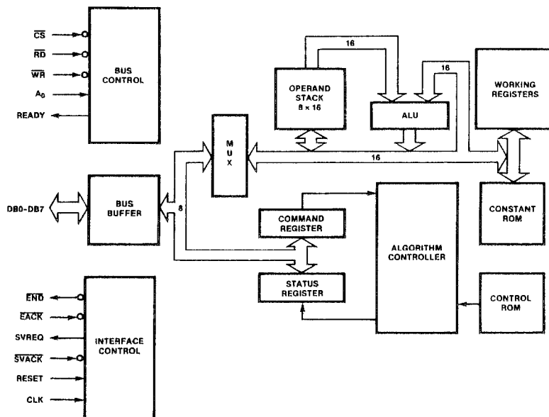
Figure 1. Block Diagram
