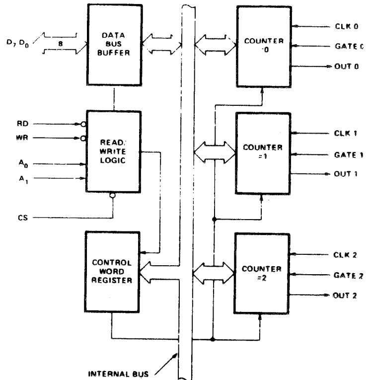
BLOCK DIAGRAM
