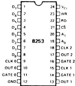
PIN CONFIGURATION
