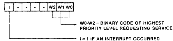
Figure 17. Poll Word
