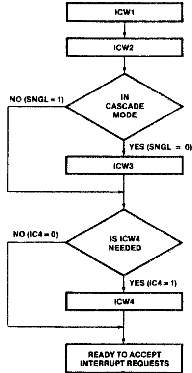
Figure 20. Initialization Flow
