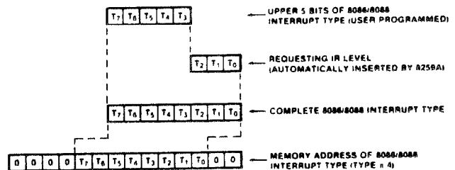
Figure 22. Establishing Memory Address of 8086/8088 Interrupt Type
