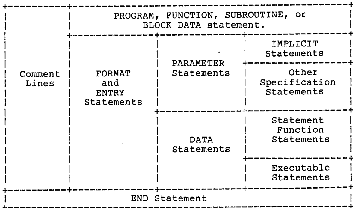
Figure 2-1: ORDERING OF LINES AND STATEMENTS IN A FORTRAN PROGRAM
