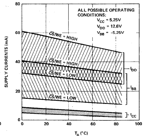
RANGE OF SUPPLY CURRENTS VS. TEMPERATURE
