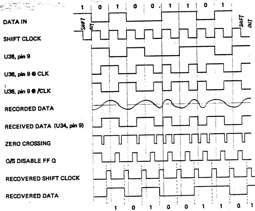
Figure 1 Timing Diagram
