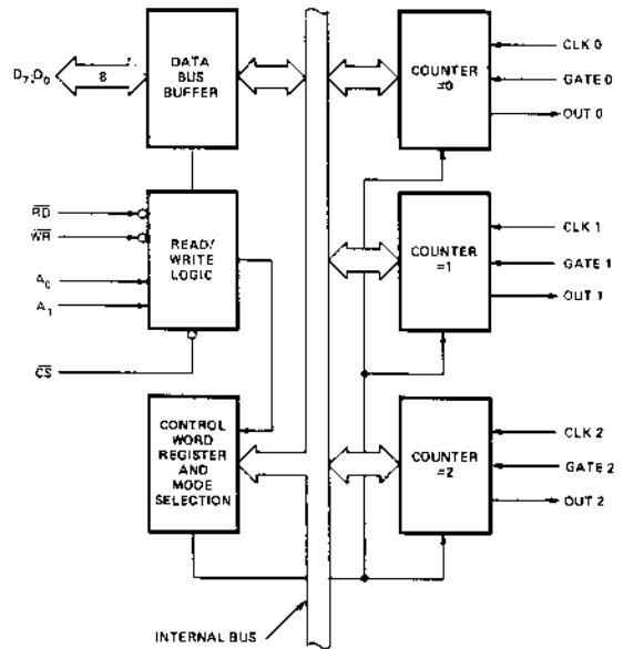
8253 Block Diagram.
