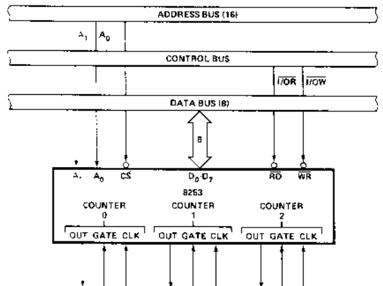
8253 System Interface.
