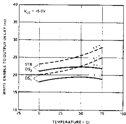
WRITE ENABLE TO OUTPUT DELAY VS. TEMPERATURE
