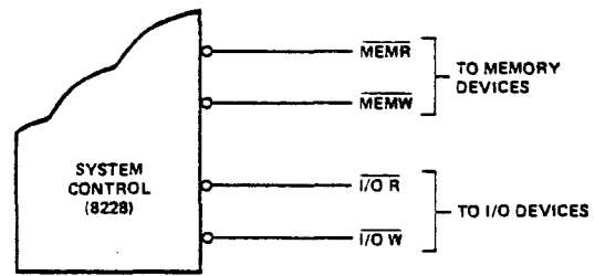
Figure 3-9. Isolated I/O.
