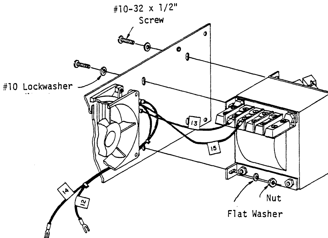
Figure 5-59. Transformer Mounting
