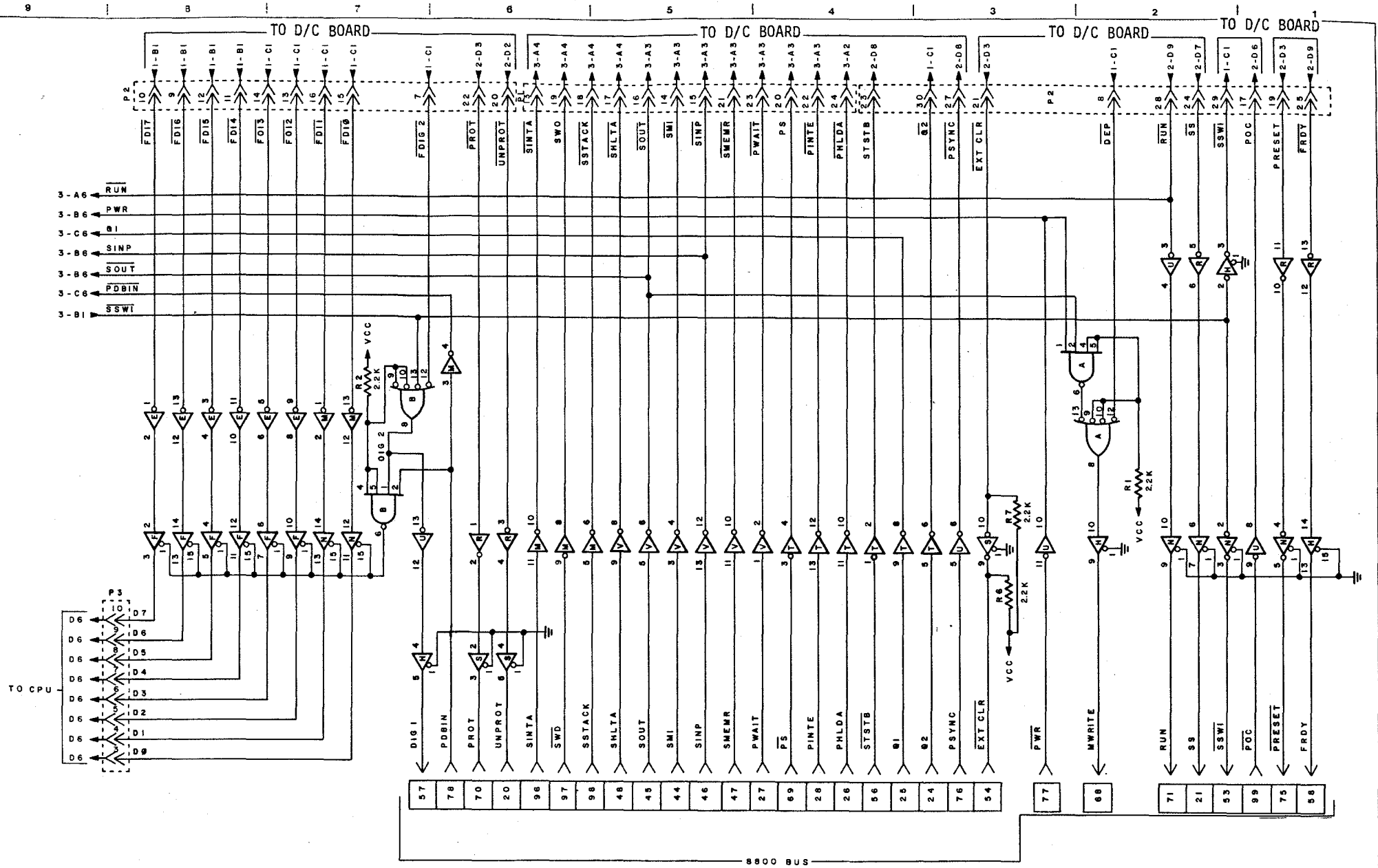
Figure 3-15. Interface Schematic (sheet 2 of 3)
