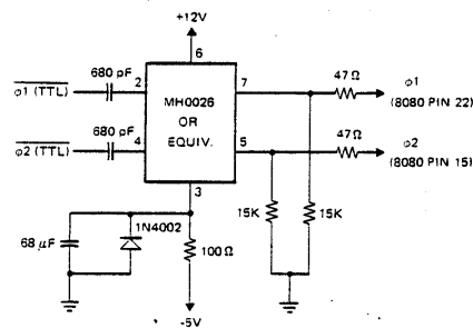
Figure 3-4. High Level Driver
