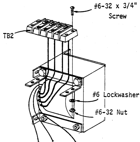
Figure 5-57. Terminal Block Mounting
