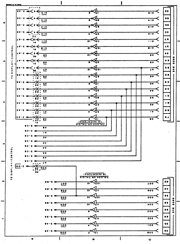
Figure 3-15. Interface Schematic (sheet 1 of 3) 3-101/(3-102 blank)
