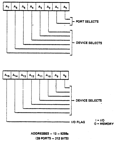
Figure 3-12. Memory Mapped I/O - (Linear Select) (8255)
