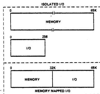
Figure 3-8. Memory/I/O Mapping.
