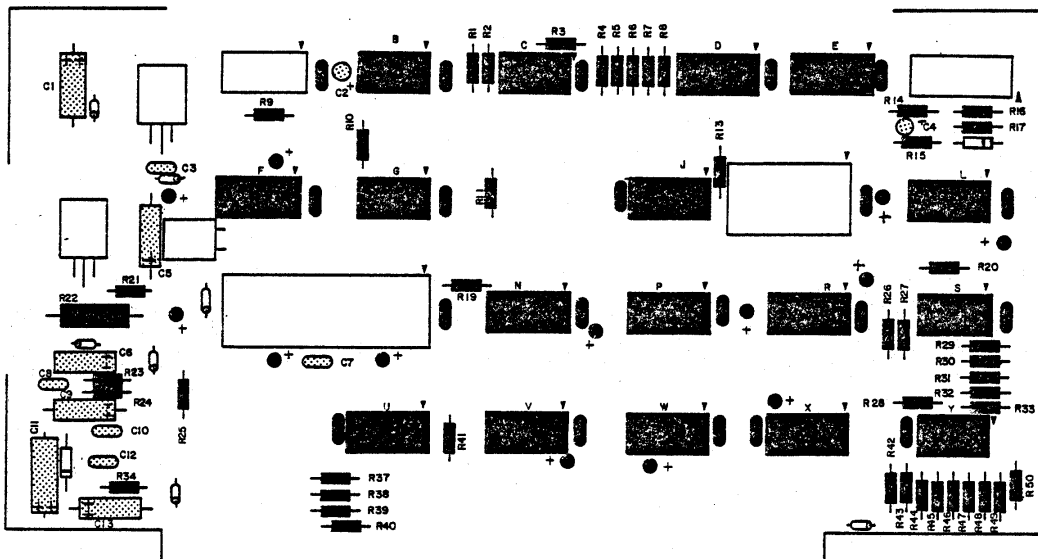
5-29. CPU Capacitor Installation
