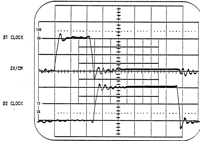
Waveform #2
