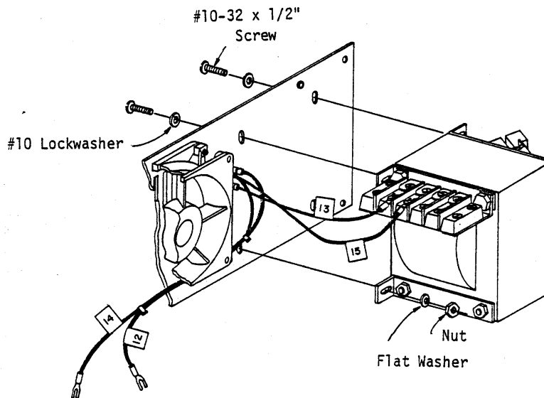
Figure 5-59. Transformer Mounting
