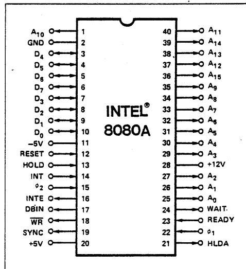
Pin Configuration
