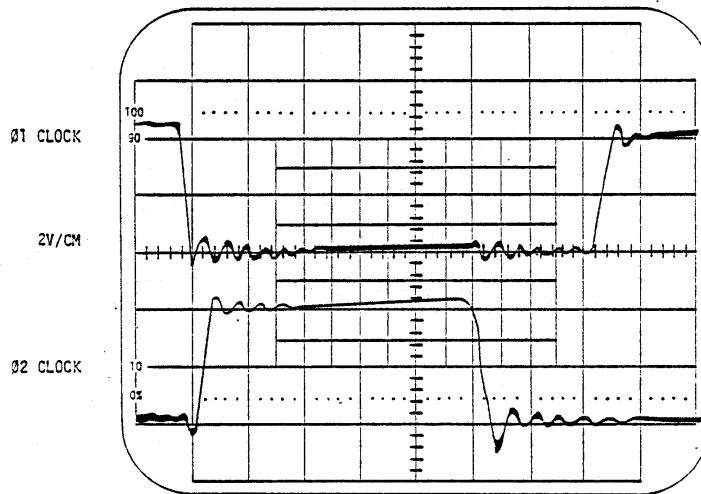
Waveform #3
