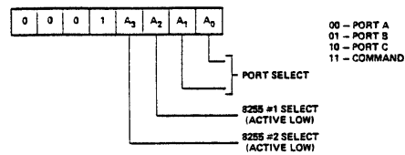
Figure 3-14. 8255 Format.
