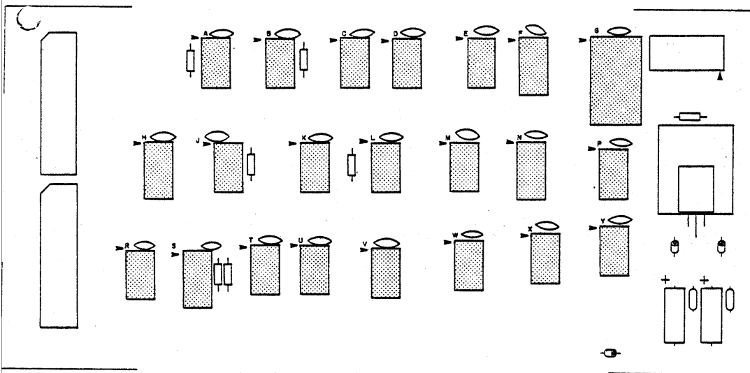
5-2. Interface IC Installation
