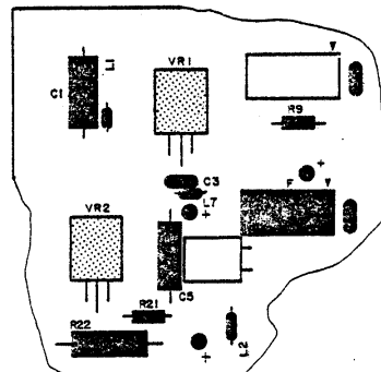
5-32. CPU Voltage Regulator Installation
