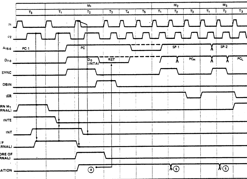
Figure 2-8. Interrupt Timing
