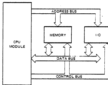
Figure 3-1. Typical Computer System Block Diagram
