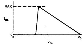
DATA BUS CHARACTERISTIC DURING DBIN
