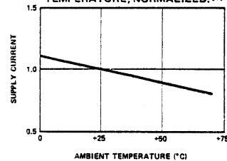
TYPICAL SUPPLY CURRENT VS. TEMPERATURE, NORMALIZED, [3]
