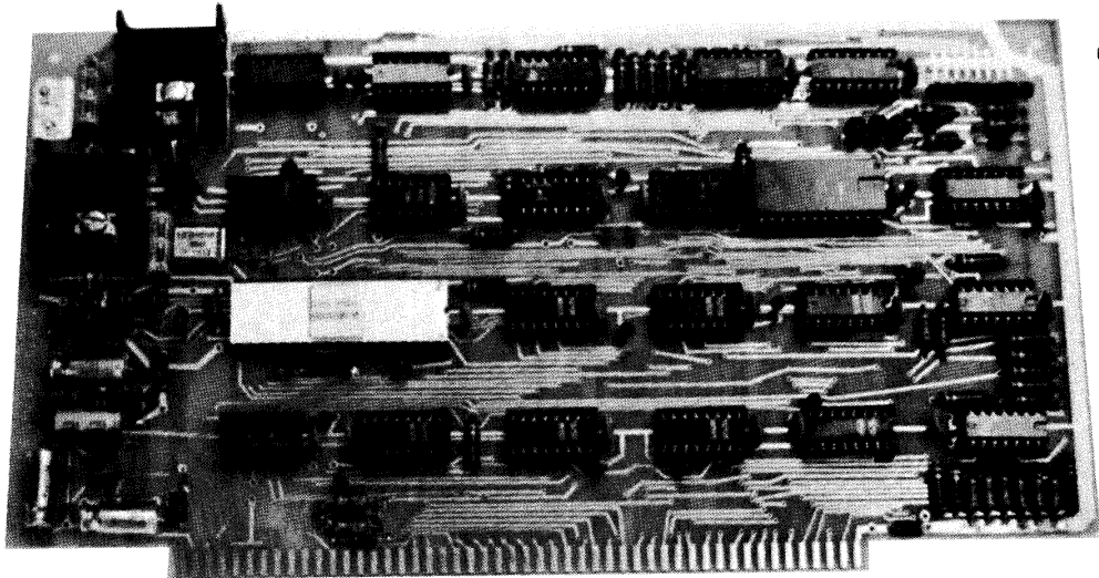
Figure 1-4. CPU Board
