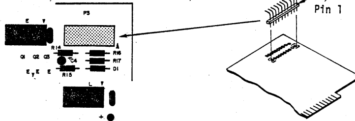
5-33. CPU Transistor and Male Connector Installation
