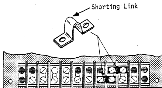
5-42. Power Supply Terminal Block Shorting Link Insertion
