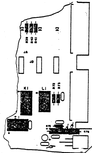
5-15. Display/Control Jumper Connections
