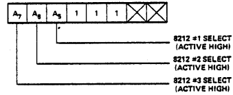
Figure 3-15. 8212 Format.
