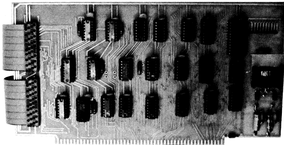
Figure 1-3. Interface Board
