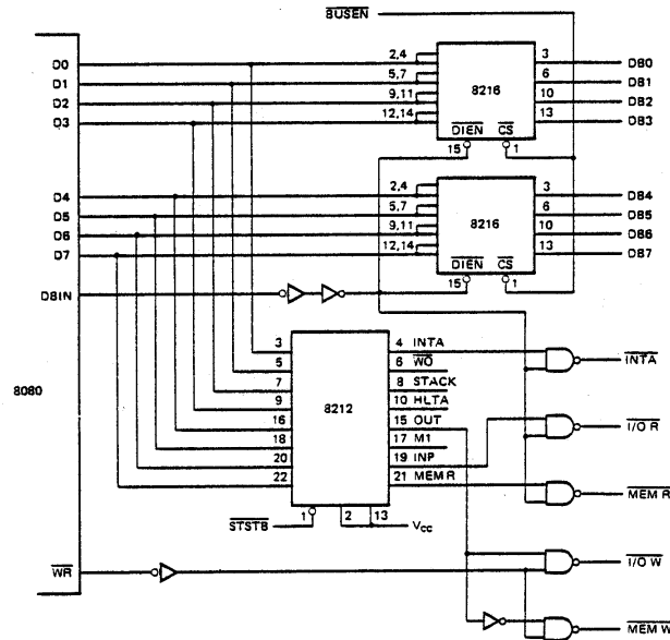
Figure 3-5. 8080 System Control
